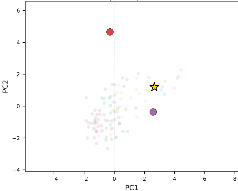
qwen3-1.7b | France
