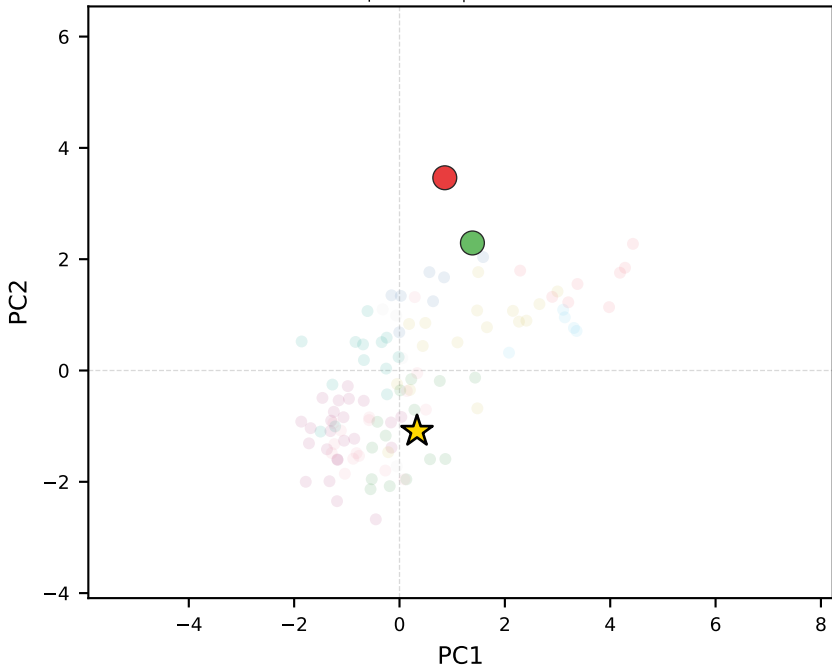
qwen3-1.7b | Guatemala
