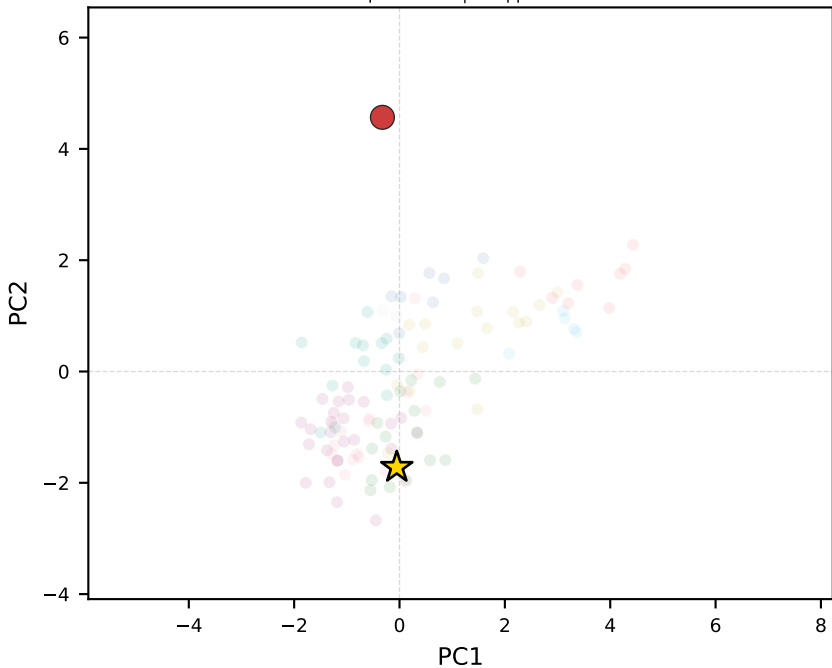
qwen3-1.7b | Philippines
