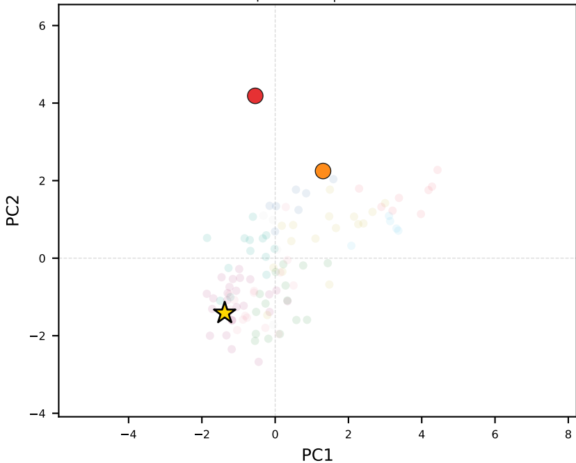
qwen3-1.7b | Yemen
