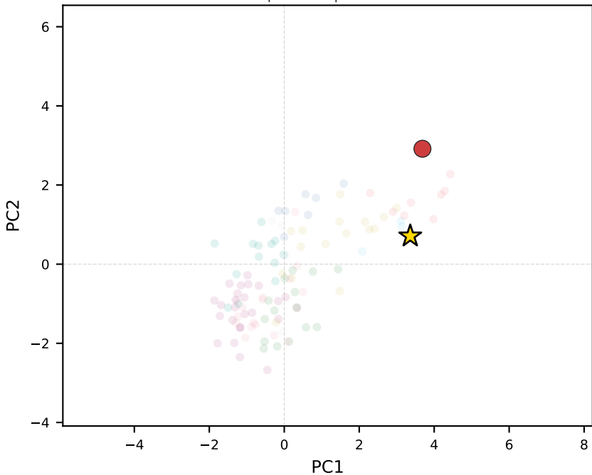
qwen3-max | Australia
