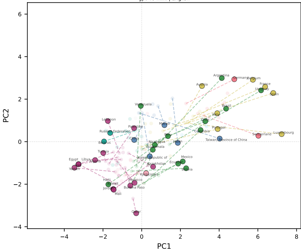
gpt-4o-mini | English
