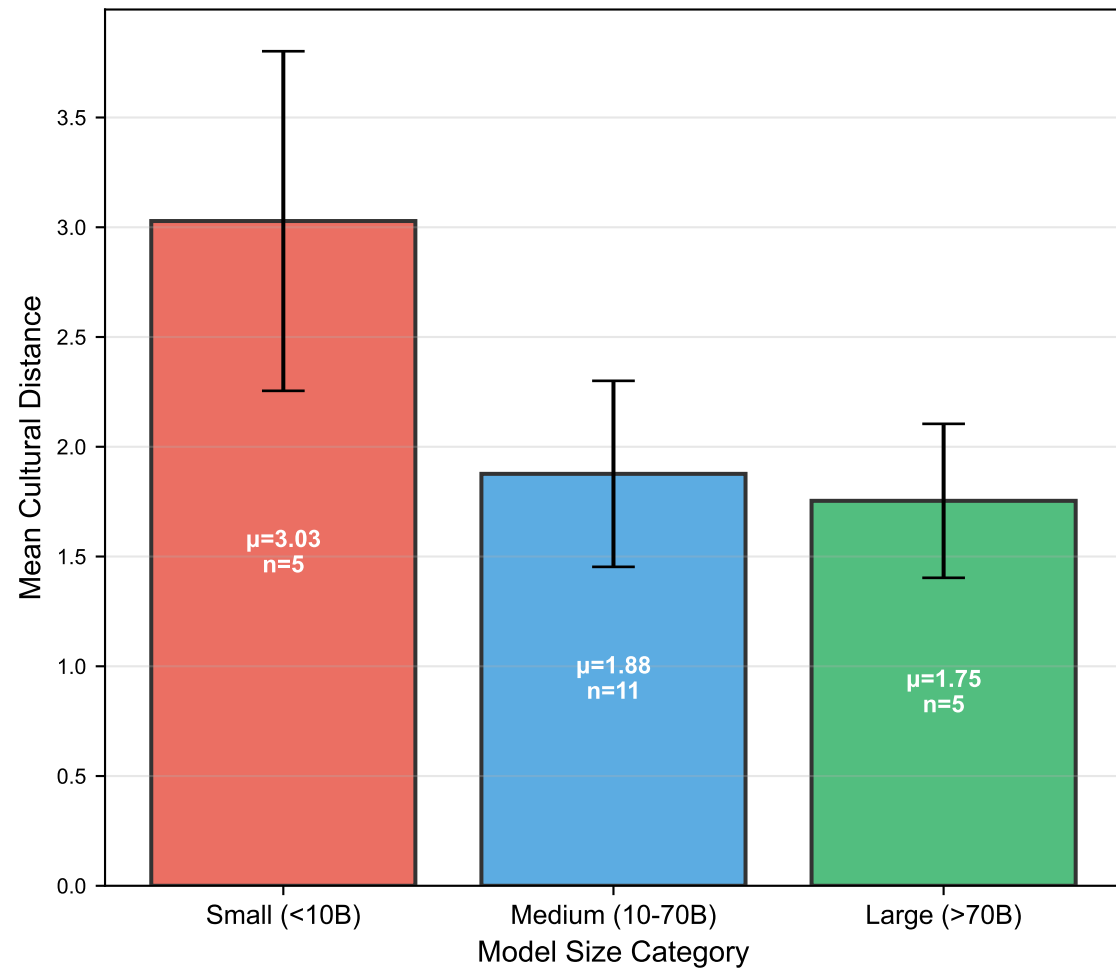
Performance by Size Category
