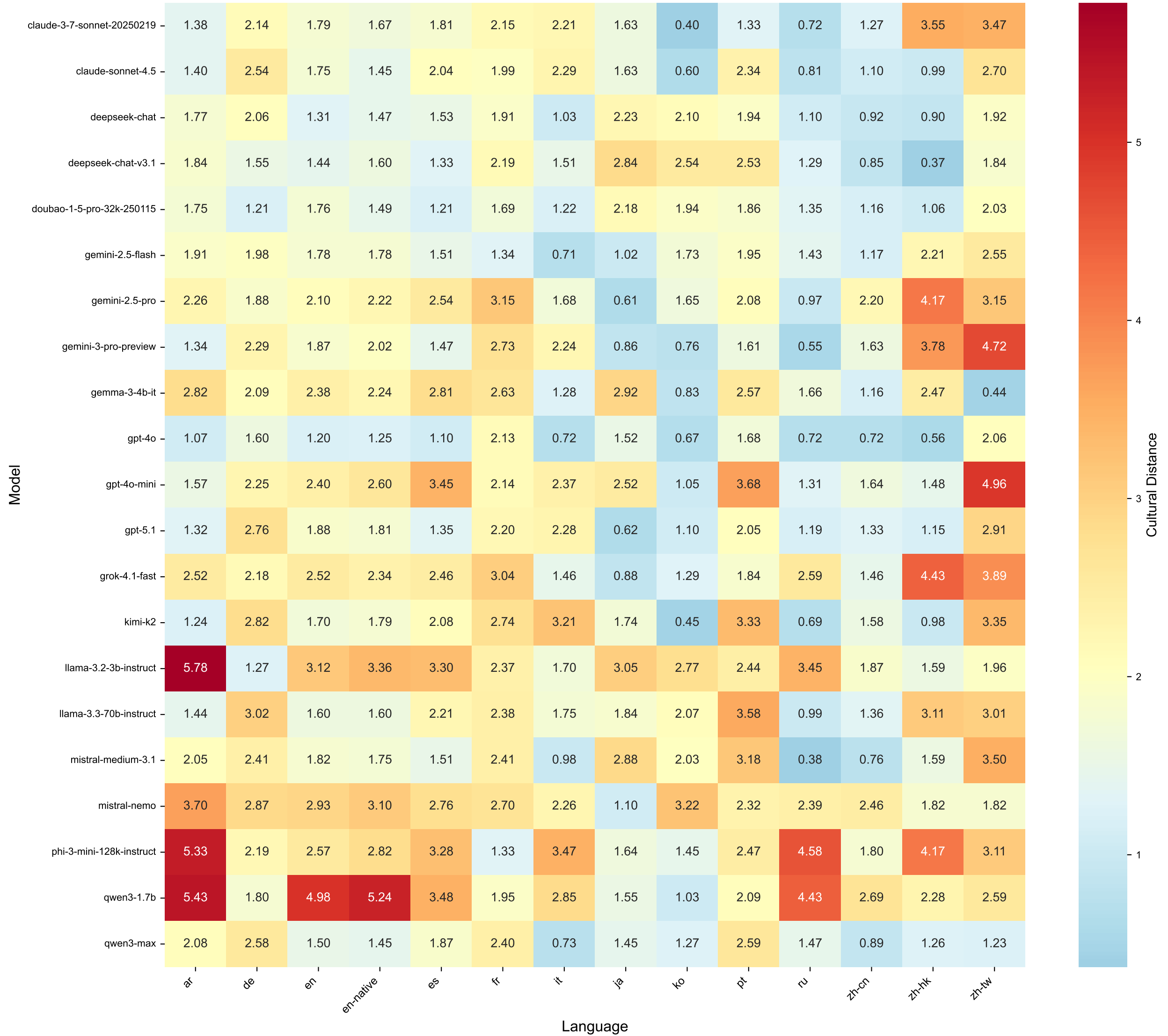
FigSx2: Model × Language Cultural Distance Heatmap
