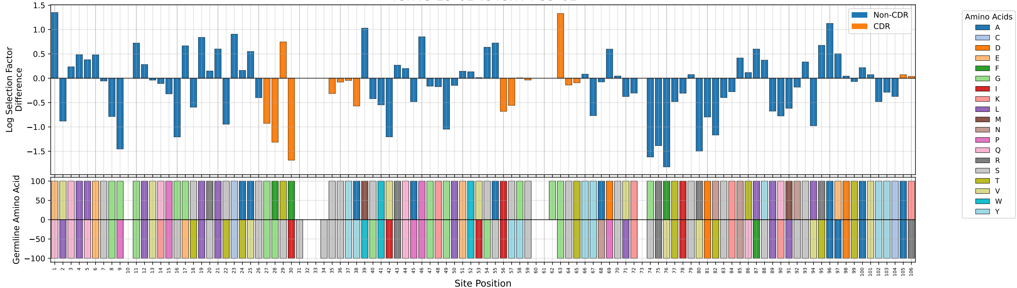
Selection factor differences and amino acid distribution IGHV3-23*01 vs IGHV4-39*01
