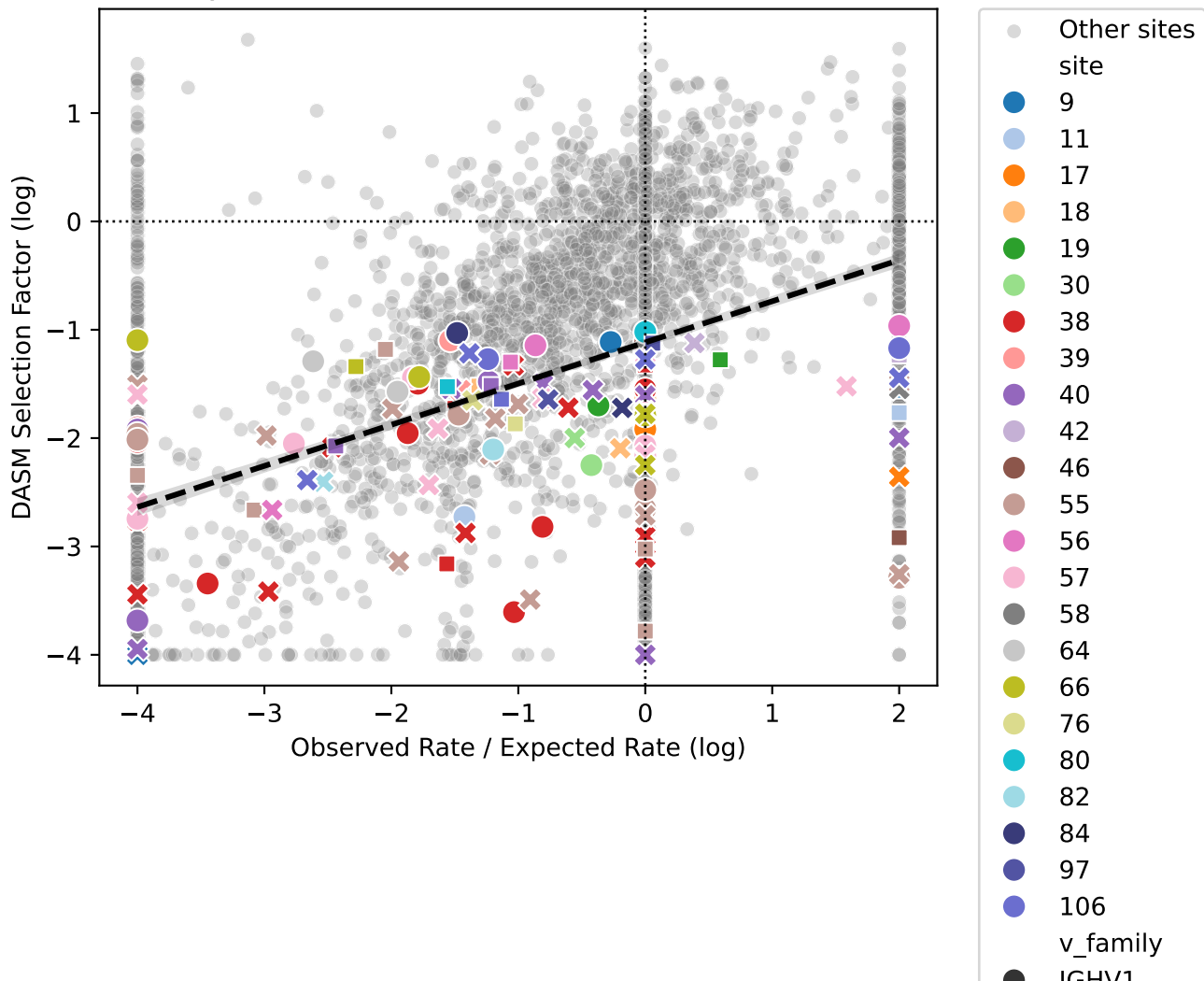
Comparison of Observed/Expected Rate Ratio vs DASM Selection Factor
