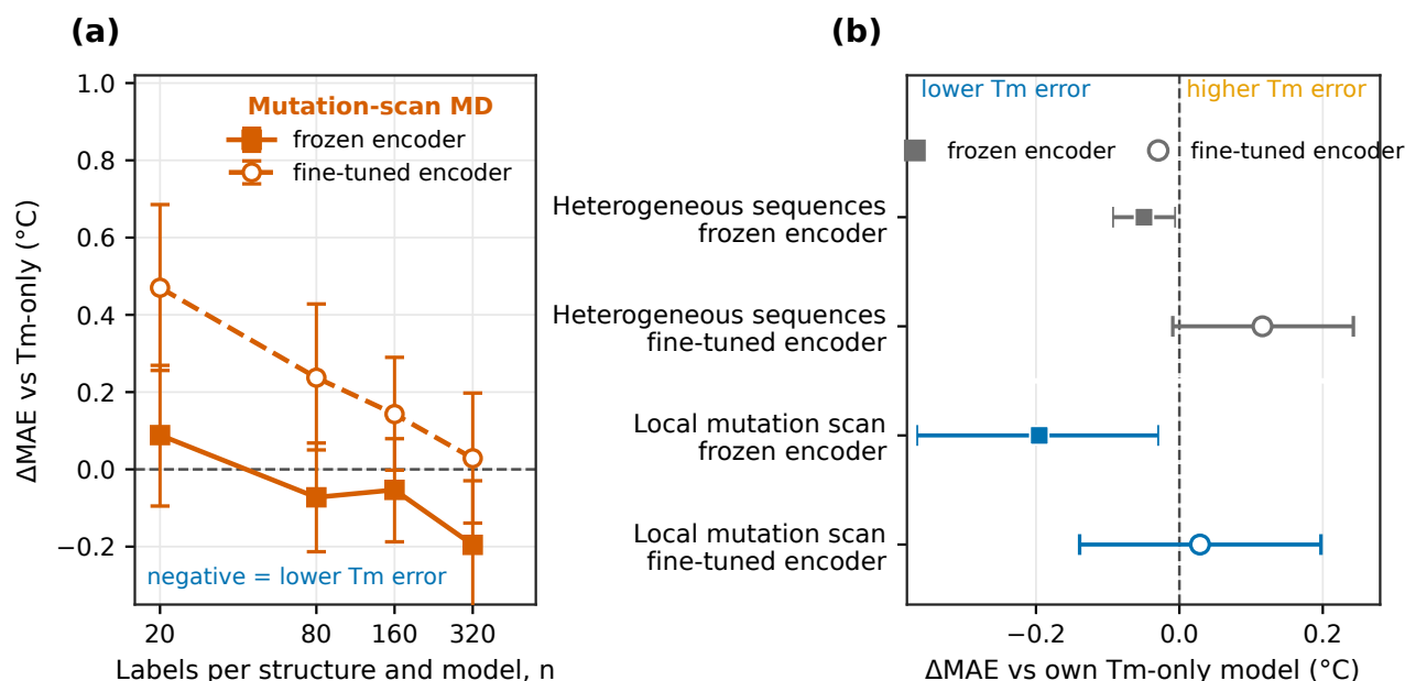
Figure 2 The MD label: label-count scaling and the variant-set contrast. (a) Paired MAE change ( \Delta\text{MAE} ) from the Tm-only baseline for the mutation-scan MD label at four label counts, with a frozen (filled, solid) and a fine-tuned (open, dashed) encoder. Here n is the number of labels sampled per structure for each ensemble member; 80% entered training. (b) \Delta\text{MAE} within each study at the largest label count, for the heterogeneous data set and the local mutation scan, with a frozen (filled) and a fine-tuned (open) encoder. Negative values mean lower Tm error after adding the MD label. Both MD data sets used the same 400 K MD and Q definition and differed only in the variants they covered; the heterogeneous data set covered nanobody structures of different lengths, whereas the mutation scans used local mutations of 1MEL and 4IDL. Predictions in (b) were averaged across ten training seeds for the heterogeneous data set and five for the mutation scans. In both panels, points and whiskers show the paired change and its 95% bootstrap interval over the 396 test sequences.
