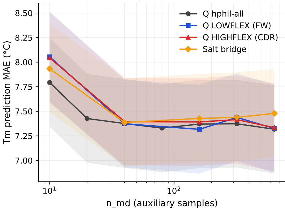
MD feature comparison (frozen ESM-2 8M)
