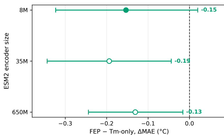
Figure S1 The FEP result held across ESM2 encoder sizes. FEP-minus-Tm-only MAE ( \Delta MAE) with a fine-tuned encoder; negative values mean lower Tm error with FEP. The 8M point is the five-seed model selected by the two-stage search, and the 35M and 650M points are ten-seed checks without size-specific tuning. Whiskers are 95% paired bootstrap intervals over the 396 Tm test sequences.
