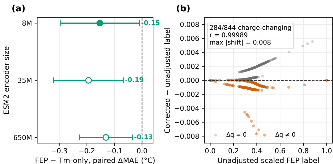
Figure S2 Robustness controls for the FEP result. (a) Paired FEP-minus-Tm-only MAE for fine-tuned ESM2 encoders. Negative values mean lower Tm error with FEP. The 8M point is the staged-selected five-seed model; the 35M and 650M points are exploratory fixed-configuration ten-seed controls and were not subjected to the same search. Whiskers are nominal 90% paired bootstrap intervals over the 396 test proteins. (b) Change in each scaled FEP label after the analytical periodic net-charge correction at dielectric 78.
