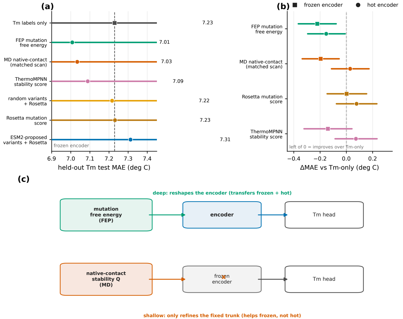
Fig. 3. Physical-observable axis: depth of transfer set by the simulated quantity. (a) Tuned frozen-encoder held-out test MAE for every source; the dashed line is the Tm-only baseline. FEP and the matched-scan MD label lead; the Rosetta-family scores sit at the baseline. (b) Paired \Delta MAE versus Tm-only for FEP, the MD native-contact label, Rosetta, and ThermoMPNN under frozen versus hot encoders; values left of zero improve on Tm-only. FEP crosses below zero in both regimes; the MD native-contact label only when frozen; Rosetta and ThermoMPNN sit near zero. (c) Interpretation: the free-energy label reshapes the shared encoder (deep; transfers frozen and hot), whereas the native-contact label only refines the fixed trunk (shallow; helps frozen, not hot). Points and intervals show ensemble MAE and 90% bootstrap intervals.
