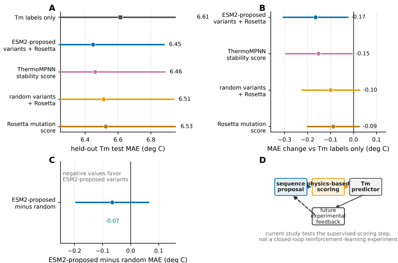
Fig. 4. Structure-based labels and language-model-proposed variants. (a) Final test MAE for Tm-only learning and non-FEP/non-MD source labels. (b) Paired \Delta MAE estimates relative to Tm-only learning. Negative values indicate improvement. (c) Direct paired comparison between ESM2-proposed variants scored by Rosetta and random variants scored by Rosetta. Negative values favor the ESM2-proposed set. (d) The result suggests a future generator–physics–predictor loop, although the present study tests only the supervised-scoring step and does not perform closed-loop optimization.
