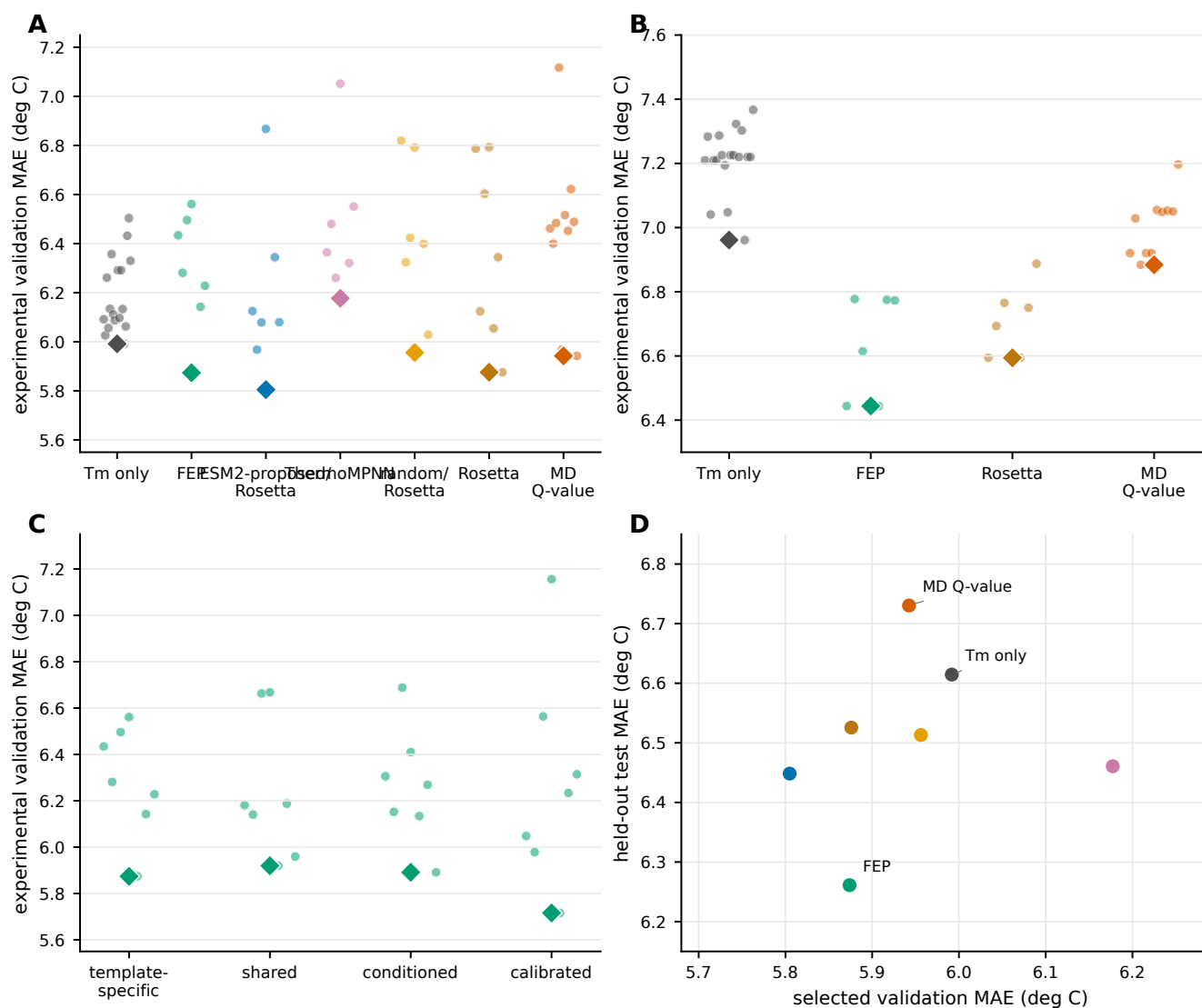
Fig. 6. Supplementary Figure 2. Candidate-setting searches and target-validation selection. (a) Experimental validation MAE values for hot-encoder source comparisons. (b) Experimental validation MAE values for frozen-encoder controls. (c) Candidate source-head designs for FEP mutation free-energy labels. (d) Relationship between selected validation MAE and held-out test MAE for the final source comparison. Diamonds mark the best validation setting in panels a–c.
