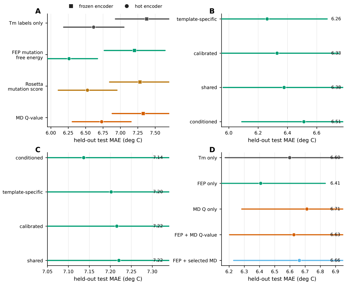
Fig. 7. Supplementary Figure 3. Model and source-combination controls. (a) Frozen-encoder and hot-encoder comparisons for selected source labels. (b) Hot-encoder FEP source-head controls. (c) Frozen-encoder FEP source-head controls. (d) Source-combination controls comparing Tm-only, FEP-only, MD-Q-only, and combined-source settings.
