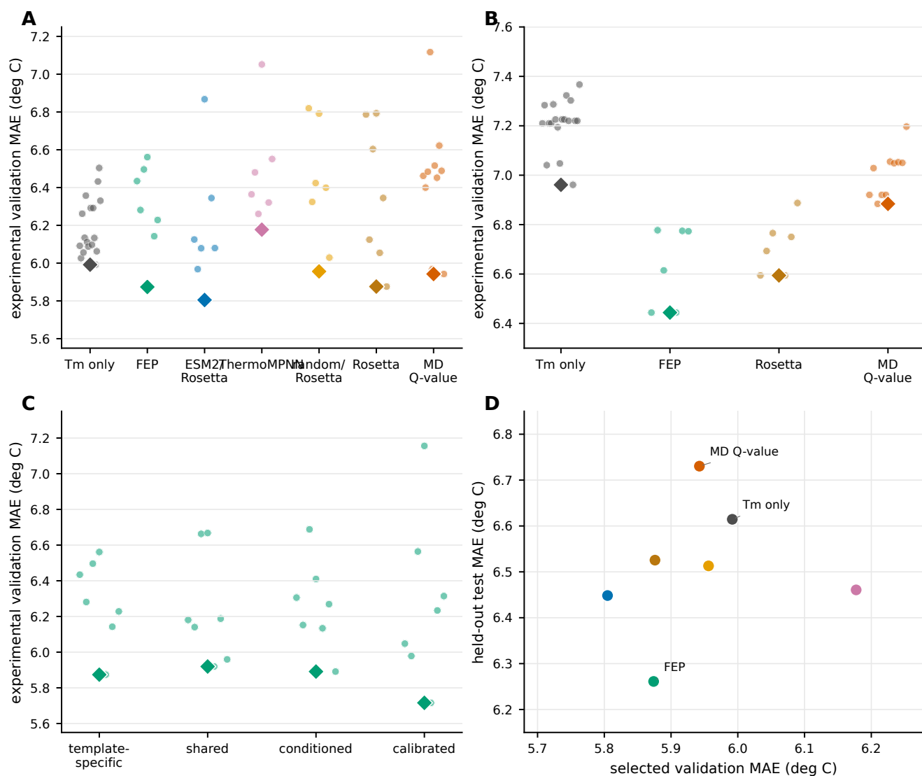
Fig. 6. Supplementary Figure 2. Candidate-setting searches and target-validation selection. (a) Experimental validation MAE values for fine-tuned-encoder source comparisons. (b) Experimental validation MAE values for frozen-encoder controls. (c) Candidate source-head designs for FEP mutation free-energy labels. (d) Relationship between selected validation MAE and held-out test MAE for the final source comparison. Diamonds mark the best validation setting in panels a–c.
