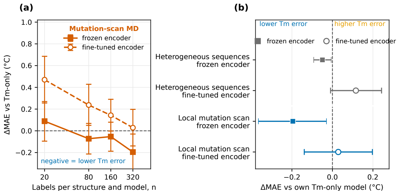
Figure 2 The MD label: label-count scaling and the variant-set contrast. (a) Paired MAE change ( \Delta\text{MAE} ) from the T_m -only baseline for the mutation-scan MD label at four label counts, with a frozen (filled, solid) and a fine-tuned (open, dashed) encoder. Here n is the number of labels sampled per structure for each ensemble member; 80% entered training. (b) \Delta\text{MAE} within each study at the largest label count, for the heterogeneous data set and the local mutation scan, with a frozen (filled) and a fine-tuned (open) encoder. Negative values mean lower T_m error after adding the MD label. Both MD data sets used the same 400 K MD and Q definition and differed only in the variants they covered; the heterogeneous data set covered nanobody structures of different lengths, whereas the mutation scans used local mutations of 1MEL and 4IDL. Predictions in (b) were averaged across ten training seeds for the heterogeneous data set and five for the mutation scans. In both panels, points and whiskers show the paired change and its 95% bootstrap interval over the 396 test sequences.
