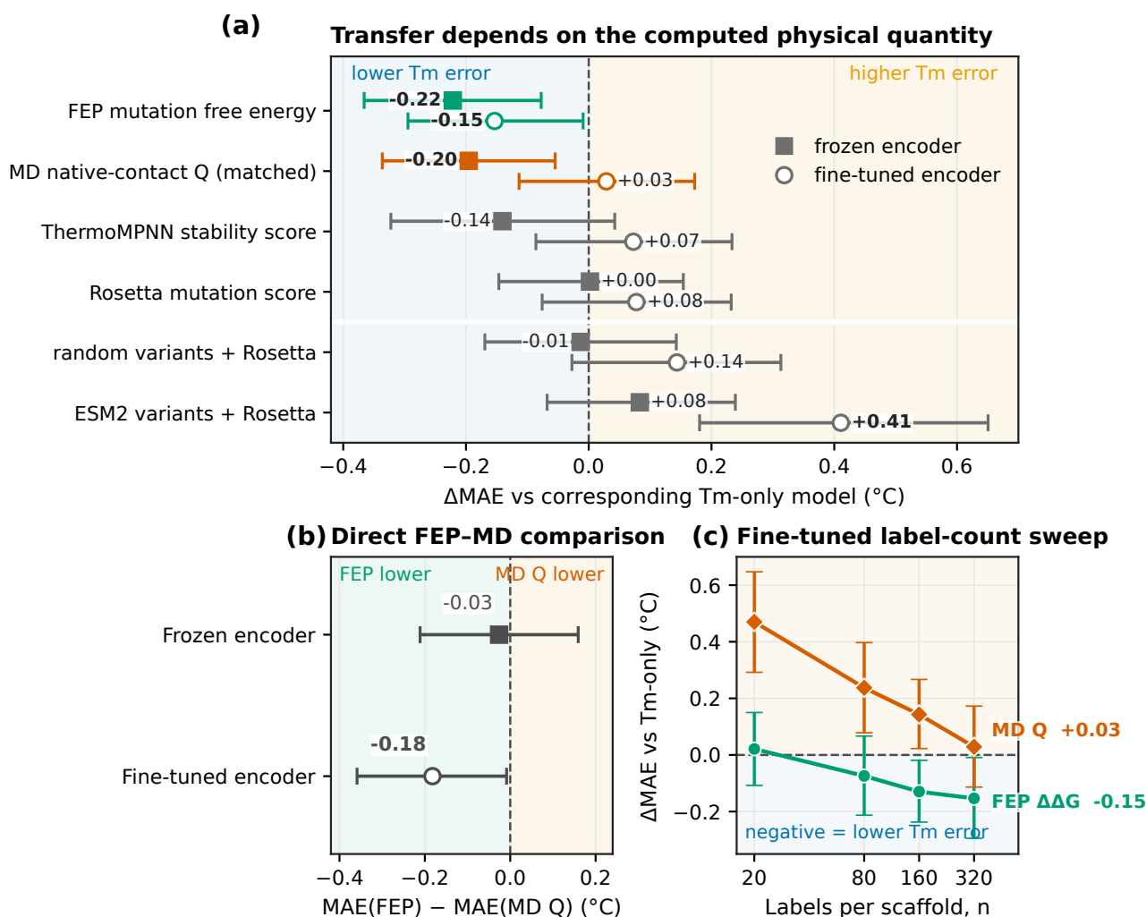
Figure 3 FEP is the only computed label that improves both encoder settings. (a) Points show the paired MAE change from the corresponding T m -only model for every tuned label. Negative values mean lower T m error. Filled squares and open circles denote frozen and fine-tuned encoders, respectively; whiskers are nominal 90% paired bootstrap intervals. Bold values have intervals that exclude zero; intervals are not adjusted for multiple comparisons. (b) Direct FEP-minus-MD comparison. Zero means equal held-out T m MAE, negative values mean lower error for FEP, and positive values mean lower error for MD native-contact Q . The bold value has a nominal 90% paired interval that excludes zero. (c) Paired MAE change from the fine-tuned T m -only model over four tested label counts on a log 2 count axis. FEP moves below zero, whereas matched MD approaches zero from higher error. Here n is the number sampled from each structure table. Whiskers are nominal 90% paired bootstrap intervals over the 396 test proteins.
