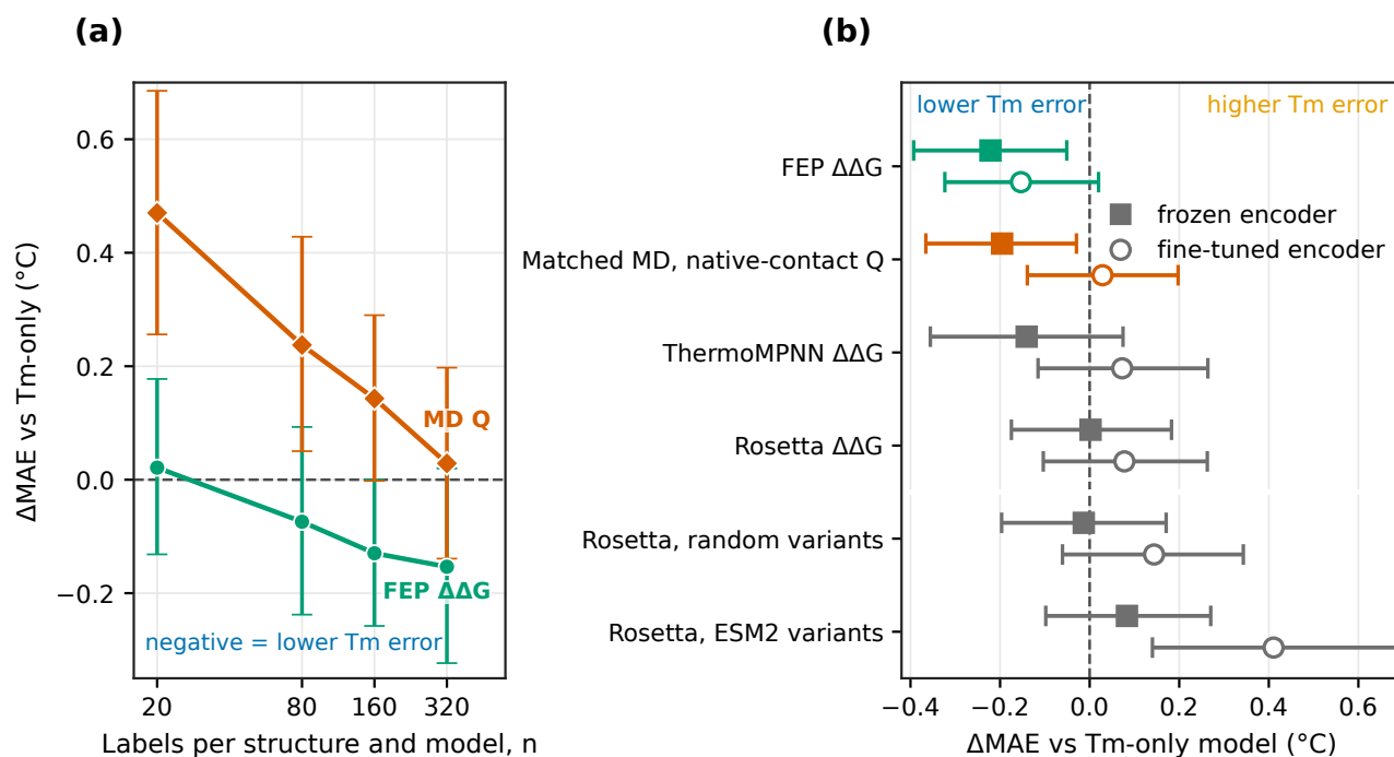
Figure 3 FEP had the lowest test Tm MAE with both encoders. (a) Paired MAE change from the fine-tuned Tm-only model for FEP and matched MD at four label counts. Here n is the number sampled from each structure for each ensemble member; 80% entered training. (b) Paired MAE change from the shared Tm-only model for each computed label. Negative values mean lower Tm error. Filled squares and open circles denote frozen and fine-tuned encoders, respectively. Whiskers in both panels are 95% bootstrap intervals over the 396 test sequences.
