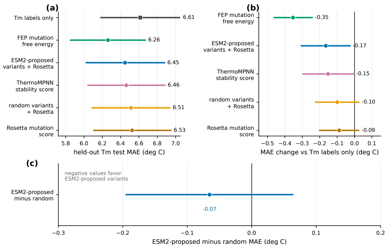
Fig. 4. Structure-based labels and language-model-proposed variants. (a) Final test MAE for Tm-only learning, FEP, and structure-based computational labels. (b) Paired \Delta MAE estimates relative to Tm-only learning. Negative values indicate improvement. (c) Direct paired comparison between ESM2-proposed variants scored by Rosetta and random variants scored by Rosetta. Negative values favor the ESM2-proposed set.
