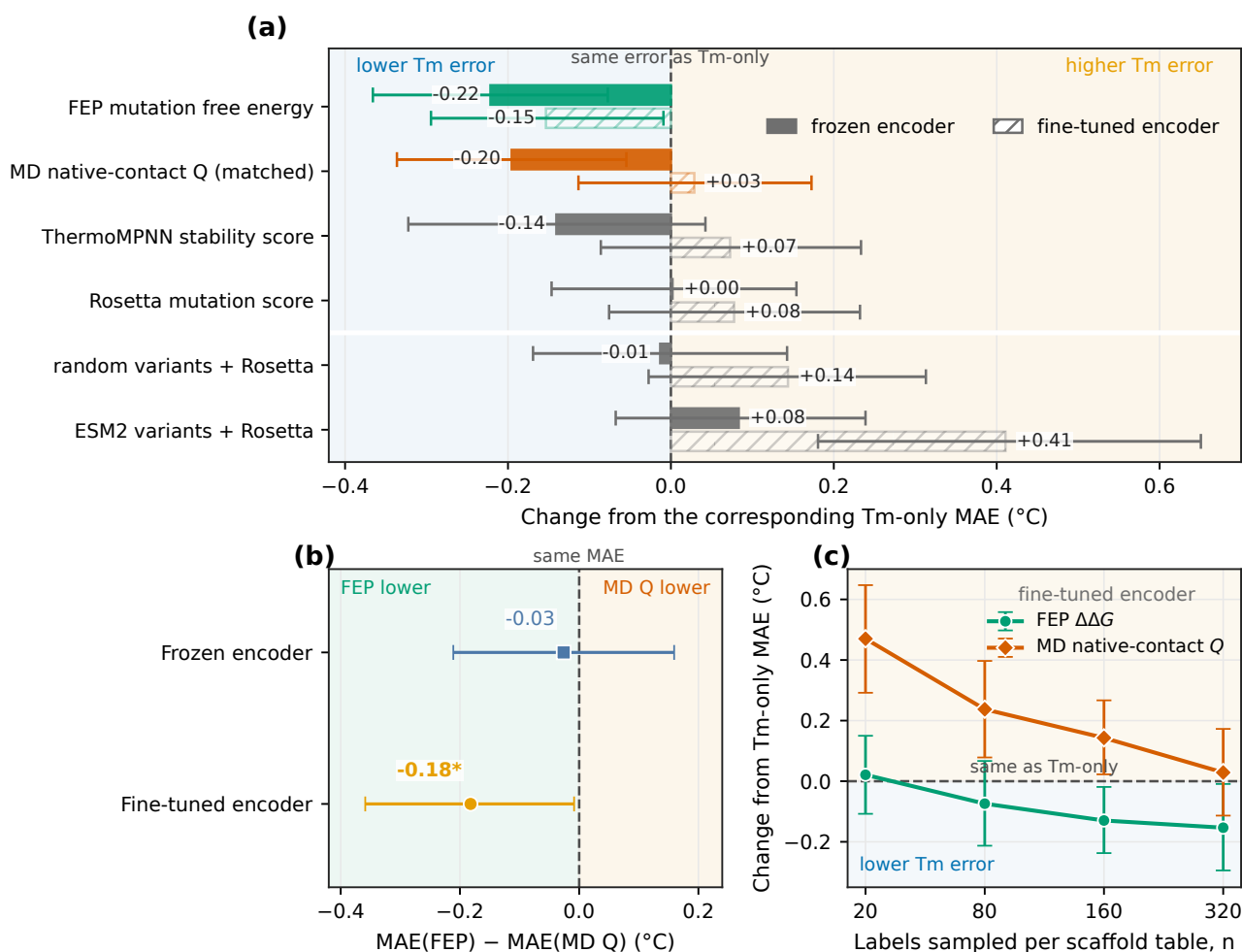
Figure 3 FEP is the only computed label that improves both encoder settings. (a) Horizontal bars show the paired MAE change from the corresponding Tm-only model for every tuned label. Negative values mean lower Tm error. Solid and hatched bars denote frozen and fine-tuned encoders, respectively; whiskers are 90% paired bootstrap intervals. (b) Direct FEP-minus-MD comparison. Zero means equal held-out Tm MAE, negative values mean lower error for FEP, and positive values mean lower error for MD native-contact Q . The asterisk marks an interval that excludes zero. (c) Paired MAE change from the fine-tuned Tm-only model over four tested label counts. FEP moves below zero, whereas matched MD approaches zero from higher error. Here n is the number sampled from each structure table. Whiskers are 90% paired bootstrap intervals over the 396 test proteins.
