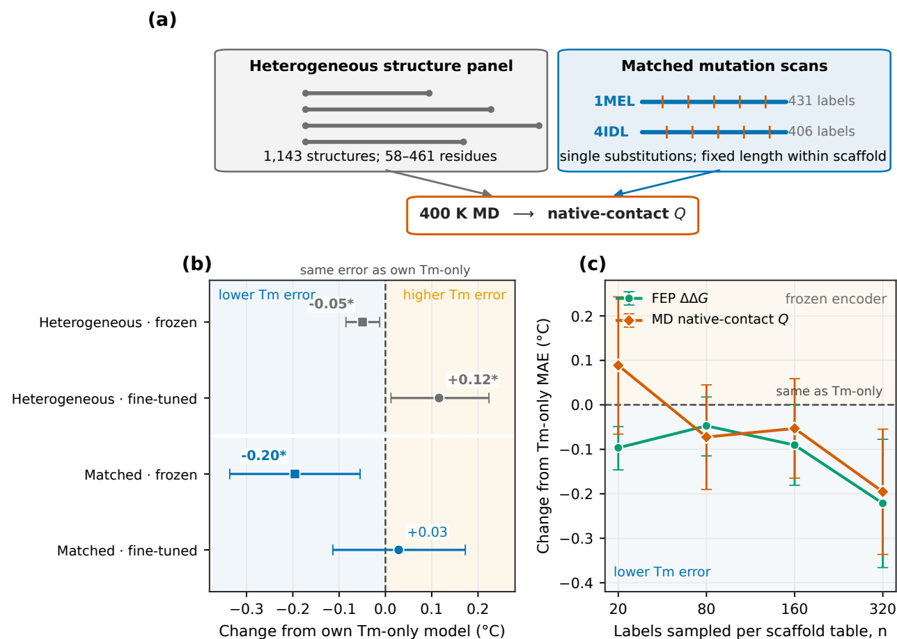
Figure 2 Matched mutation scans show a larger frozen-encoder gain from native-contact Q . (a) A heterogeneous structure panel and local mutation scans on the fixed 1MEL and 4IDL structures use similar simulation time per sequence and produce labels from the same Q family. The complete pipelines also differ in contact selection and averaging windows. (b) Paired MAE change for each simulation plan and encoder setting. Zero means equal MAE to that series' own Tm-only model, and negative values mean lower Tm error. Because the two series were tuned independently, their absolute MAEs are not compared. Asterisks mark 90% paired bootstrap intervals that exclude zero. (c) Paired MAE change from the frozen Tm-only model over four tested label counts. Here n is the number sampled from each structure table. Points and whiskers show the paired change and its 90% bootstrap interval over the 396 test proteins.
