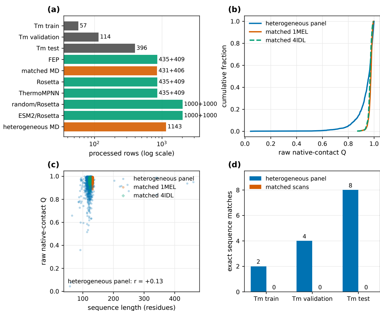
Figure 1 Data sets and diagnostics for the two MD acquisition plans. (a) Processed row counts. Labels of the form a + b give the 1MEL and 4IDL table sizes. (b) Empirical cumulative distributions of the raw native-contact Q values for the heterogeneous structure panel and the two matched mutation scans. The extraction details are not identical, so the distributions are descriptive. (c) Raw Q versus sequence length. The matched scans have one fixed length per structure, whereas the heterogeneous panel spans 58–461 residues and has Pearson r = +0.13 . (d) Exact sequence matches to the three NbBench splits. The matched scans have no matches; the heterogeneous panel has 2, 4, and 8.
