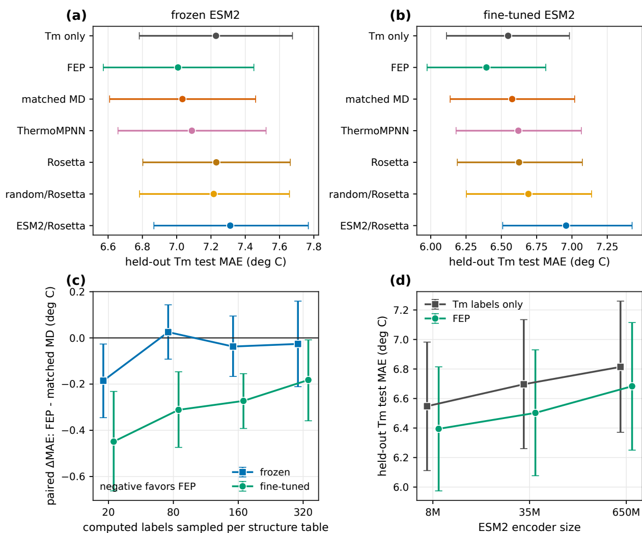
Figure 3 Absolute test errors and transfer controls. (a,b) Held-out Tm test MAE for every selected source with frozen and fine-tuned ESM2. Whiskers are 90% bootstrap intervals over the 396 test proteins. (c) Direct paired difference between FEP and matched-MD absolute errors at each label count. Negative values favor FEP; whiskers are 90% paired bootstrap intervals. (d) Available fine-tuned ESM2-size controls for Tm-only and FEP models. Increasing encoder size did not reproduce the 8M FEP result.
