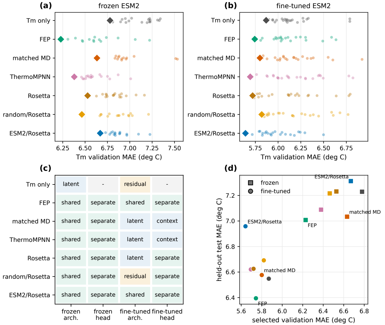
Figure 2 Per-source model selection using experimental Tm validation data. (a,b) Stage-2 candidate validation MAEs for frozen and fine-tuned ESM2. Each small point is one candidate; diamonds mark the selected setting. No test errors enter this selection. (c) Architecture and computational-head form selected for every source and encoder setting. A dash denotes a Tm-only model without a computational head. (d) Selected validation MAE and the later held-out test MAE. Colors match panels a and b; squares and circles denote frozen and fine-tuned ESM2.
