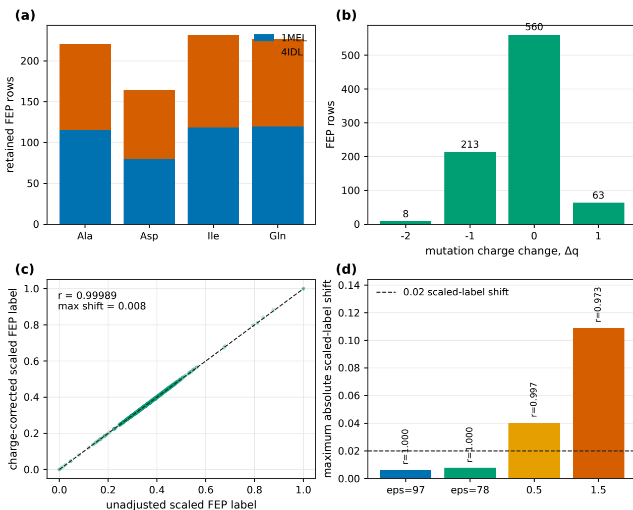
Figure 4 Provenance and charge-change checks for the retained FEP labels. (a) Rows from the retained Ala, Asp, Ile, and Gln scans, separated by structure. (b) Distribution of formal mutation charge changes. (c) Model-facing FEP labels before and after the analytical periodic net-charge correction at dielectric 78. The dashed line is equality. (d) Maximum scaled-label shift under two periodicity estimates and two larger sensitivity values in kcal mol -1 per ( \Delta q ) 2 . Numbers above the bars give the corrected-versus-uncorrected correlation. The larger values are sensitivity bounds, not estimates of omitted correction terms.
