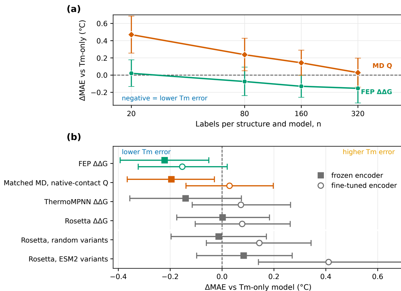
Figure 3 FEP had the lowest test Tm MAE with both encoders. (a) Paired MAE change from the fine-tuned Tm-only model for FEP and matched MD at four label counts. Here n is the number sampled from each structure for each ensemble member; 80% entered training. (b) Paired MAE change from the shared Tm-only model for each computed label. Negative values mean lower Tm error. Filled squares and open circles denote frozen and fine-tuned encoders, respectively. Whiskers in both panels are 95% bootstrap intervals over the 396 test sequences.
