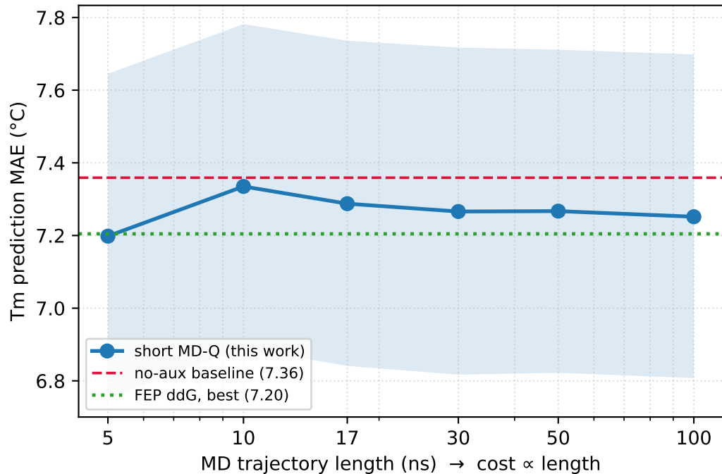
frozen encoder ( n_{md}=640 )
