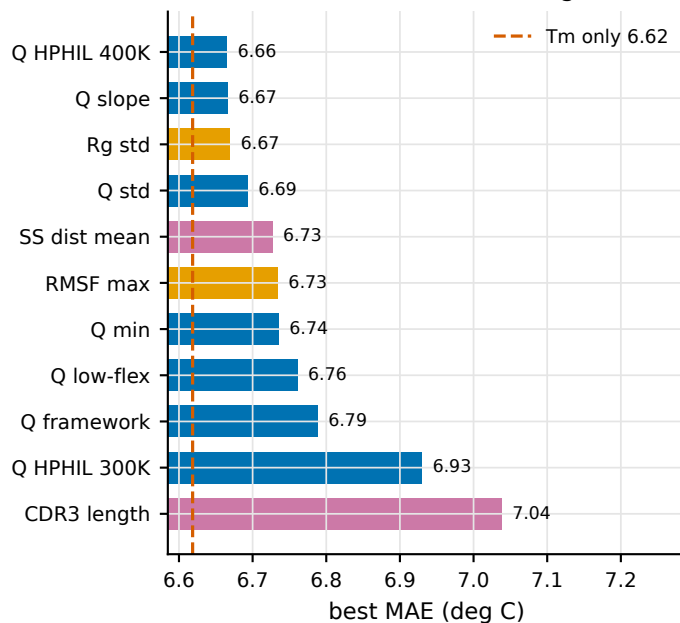
D Encoder effect by feature
