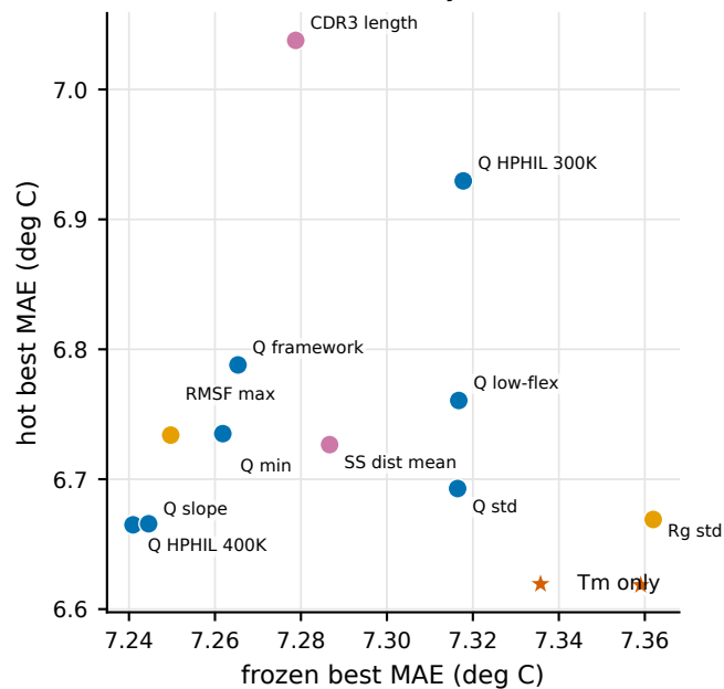
D Encoder effect by feature
