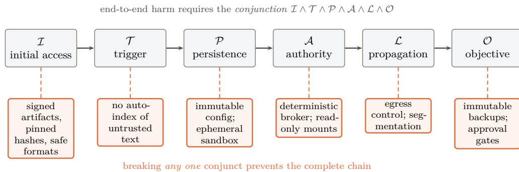
Figure 19.1: The defender’s arithmetic. Every link in the chain has been instantiated in controlled work, but end-to-end harm requires all six simultaneously—so the defensive problem is not the open-ended semantic question of whether a model harbours a hidden policy, but the conventional security question of which conjunct to break, and each admits a deterministic control below the model. After the companion survey [291]; see Table 19.1 for the evidence status of each condition.
