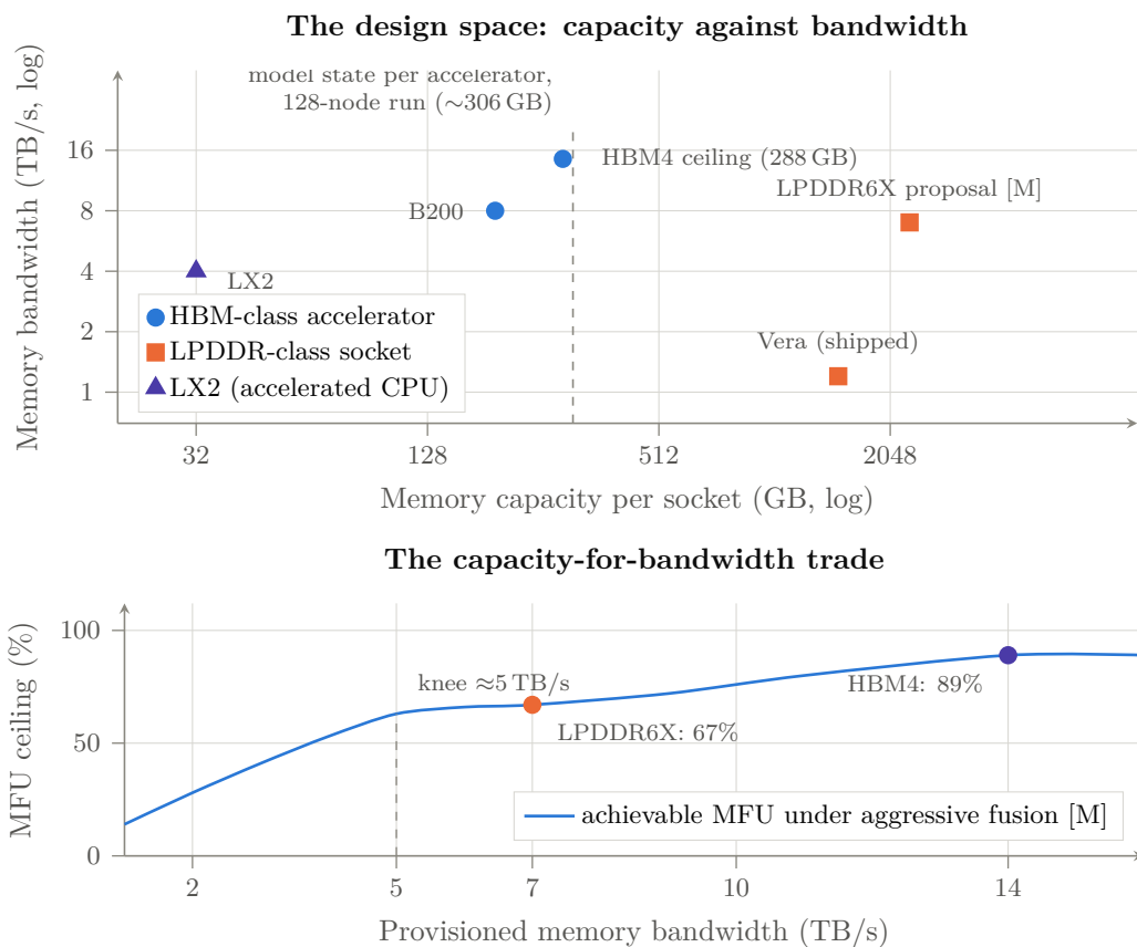
Figure 12.2: Why capacity is the arbitrage. Above : capacity against bandwidth for shipped parts [V] and for the modeled LPDDR6X socket [M]. The dashed line is the per-accelerator model state for the reference 2.8T-parameter sparse-MoE run at 128 nodes ( \sim 306 \text{ GB} ): everything to its left cannot hold the model at all, which is the sense in which the HBM path has a cluster-size floor. Below : the trade the substitution buys—22 points of MFU ceiling surrendered for an eightfold capacity gain and an order-of-magnitude better cost per bit. Curve shape is modeled, not measured; Appendix A states the experiments that would confirm or refute it.
