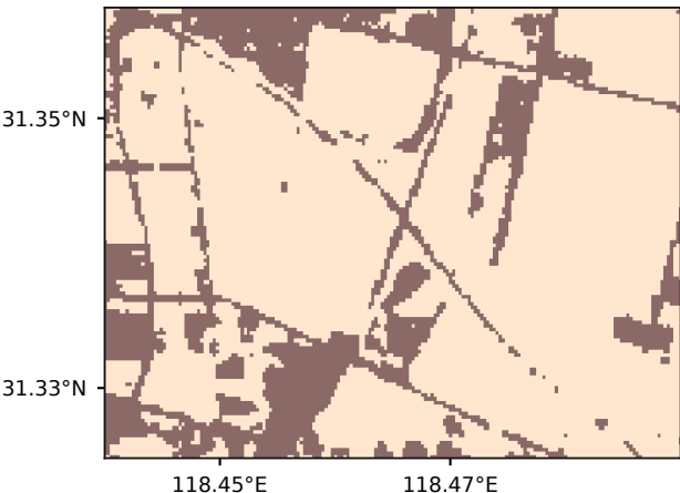
(c) NESDC rice, 10 m
