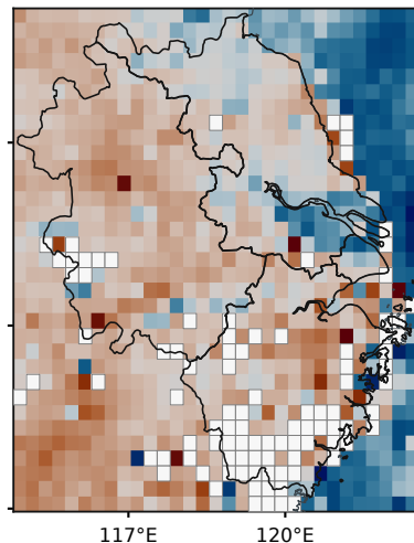
(c) observed minus that field
