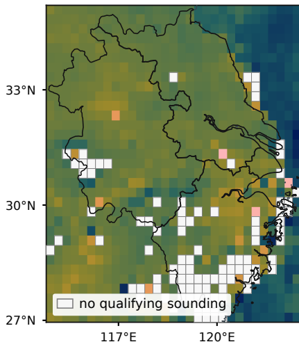
(a) observed methane, 2018 annual mean
