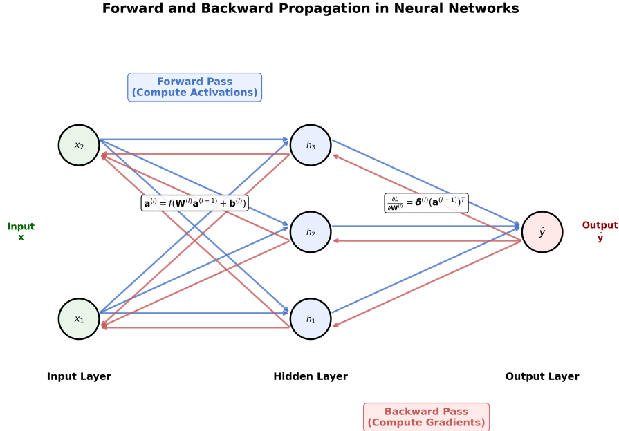
Figure 2.2: Gradient flow illustration showing backpropagation through a neural network. Forward pass (blue arrows) computes activations, while backward pass (red arrows) propagates gradients for parameter updates.
