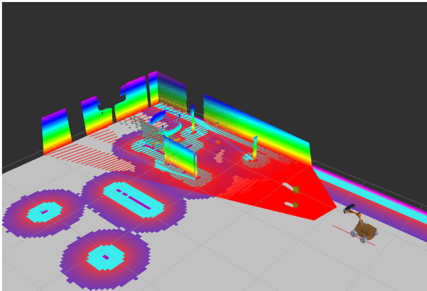
Figure 16: The point cloud as received from the camera topic including the eventual bounding boxes
