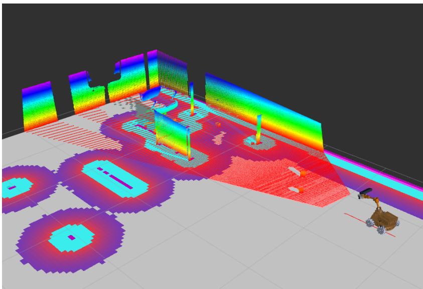
Figure 17: The downsampled point cloud
