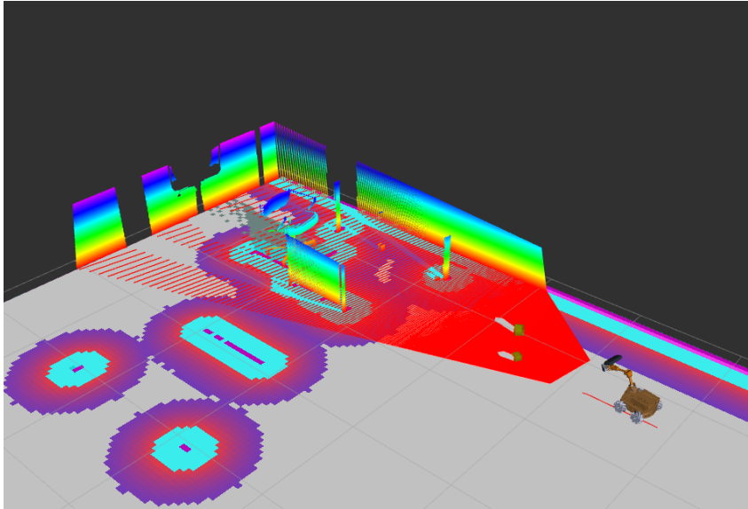
Figure 16: The point cloud as received from the camera topic
