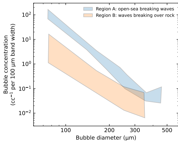
Bubble concentration ( \text{cc}^{-1} per 100 \mu\text{m} band width) in seawater produced by breaking waves. Shaded regions show bubble concentrations from different wave conditions: breaking waves on the open sea (Region A) and waves breaking over a rock (Region B), demonstrating the variability in bubble production mechanisms. Redrawn from data digitised from Figure 4 of Blanchard and Woodcock [1957] under CC BY ( https://doi.org/10.3402/tellus.v9i2.9094 ).
