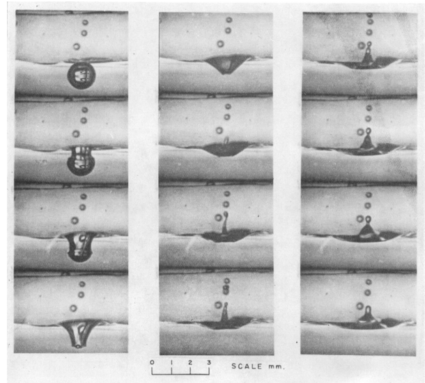
High-speed motion pictures of bubble bursting dynamics, reproduced from Kientzler et al. [1954] under CC BY ( https://doi.org/10.3402/tellus.v6i1.8717 ). Sequence shows 1.5 mm diameter bubbles bursting in fresh water with a clean surface, captured horizontally through a glass microscope slide. The images were taken at 3,340 frames per second, revealing the progressive stages of bubble cavity collapse and jet formation.
