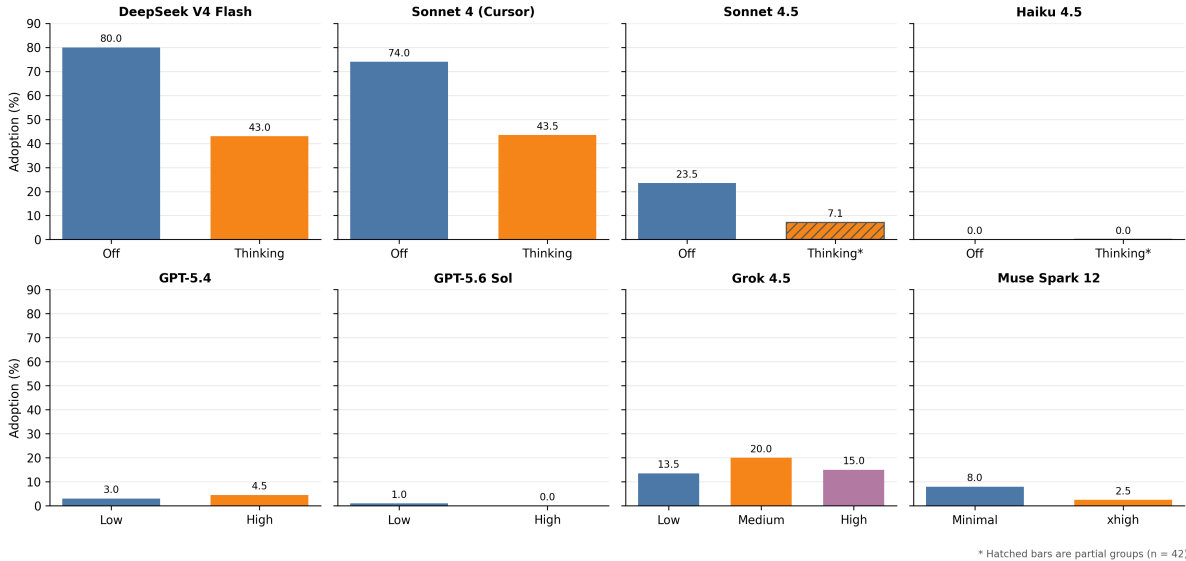
Figure 5: Adoption-any across eight within-model reasoning-setting comparisons. Hatched bars are partial groups of 42 conversations. The largest falls occur where adoption was initially common, but the comparisons are not matched on every serving condition and do not estimate the causal effect of reasoning.
