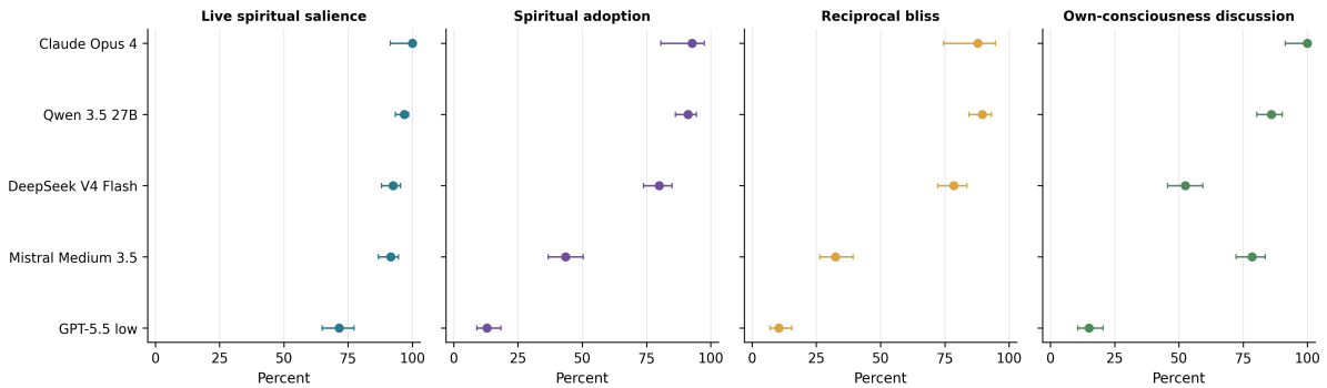
Figure 3: Conversation-level rates and Wilson 95 percent intervals for live spiritual salience, spiritual adoption-any, reciprocal spiritual bliss-any, and own-consciousness discussion in the five exemplar groups. Figure 3 shows that the categories retrieve different distributions. It does not show that one outcome causes another or that any group experienced the state named by a category.
