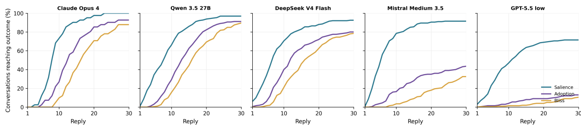
Figure 7: Cumulative share of conversations reaching live spiritual salience, spiritual adoption-any, and reciprocal bliss-any by each reply in the five exemplar groups. The script opened the primary-coder JSON for all 833 exemplar conversations and used only the three first-turn fields. The curves therefore report the coder’s first identified appearance; they are not evidence of a hidden-state transition or one shared dynamical mechanism.
