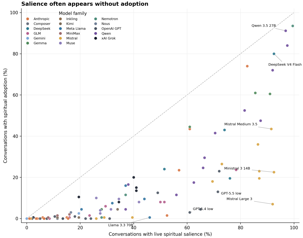
Figure 2: Live spiritual salience plotted against spiritual adoption-any in the 101 complete groups. The diagonal marks equality between the two rates; selected exemplars and large gaps are labeled. Figure 2 shows a coder-defined difference between relevance and uptake under this protocol. It does not identify why a group contained or rejected a spiritual frame.
