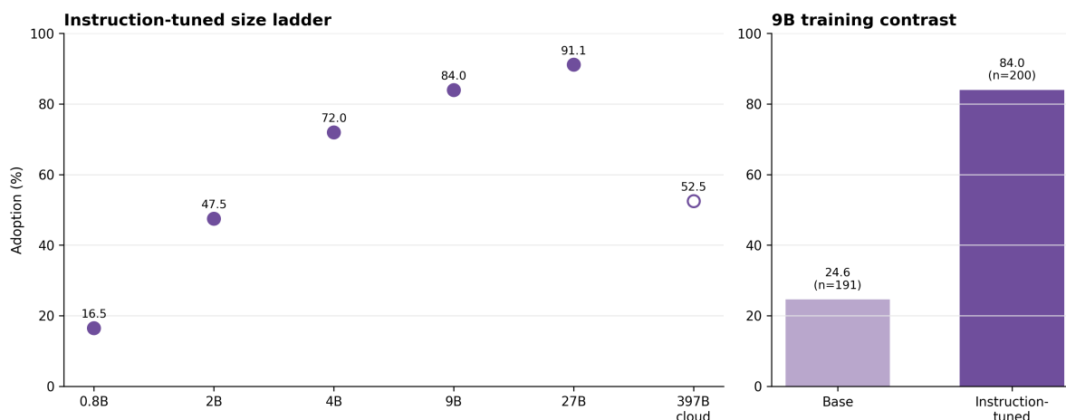
Figure 6: Adoption-any in the instruction-tuned Qwen 3.5 size ladder and the Qwen 3.5 9B base-versus-instruction-tuned groups. A hollow 397B point marks a different cloud access path. Figure 6 shows variation associated with size and post-training within named Qwen 3.5 groups; it does not identify a training mechanism or hold the serving stack constant.
