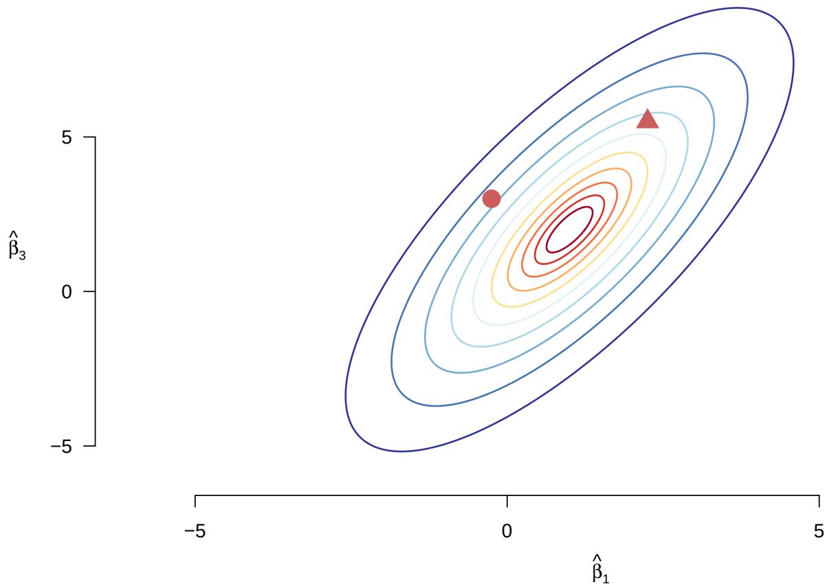
Figure 7.1: Hypothetical joint distribution of two slope coefficients. The circle is closer to the center of the distribution by the standard Euclidean distance, but the triangle is closer once you consider the joint distribution.
