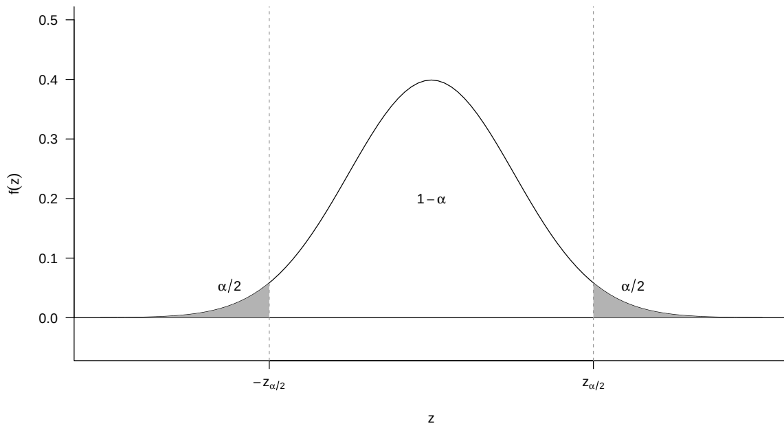
Figure 3.3: Critical values for the standard normal.
