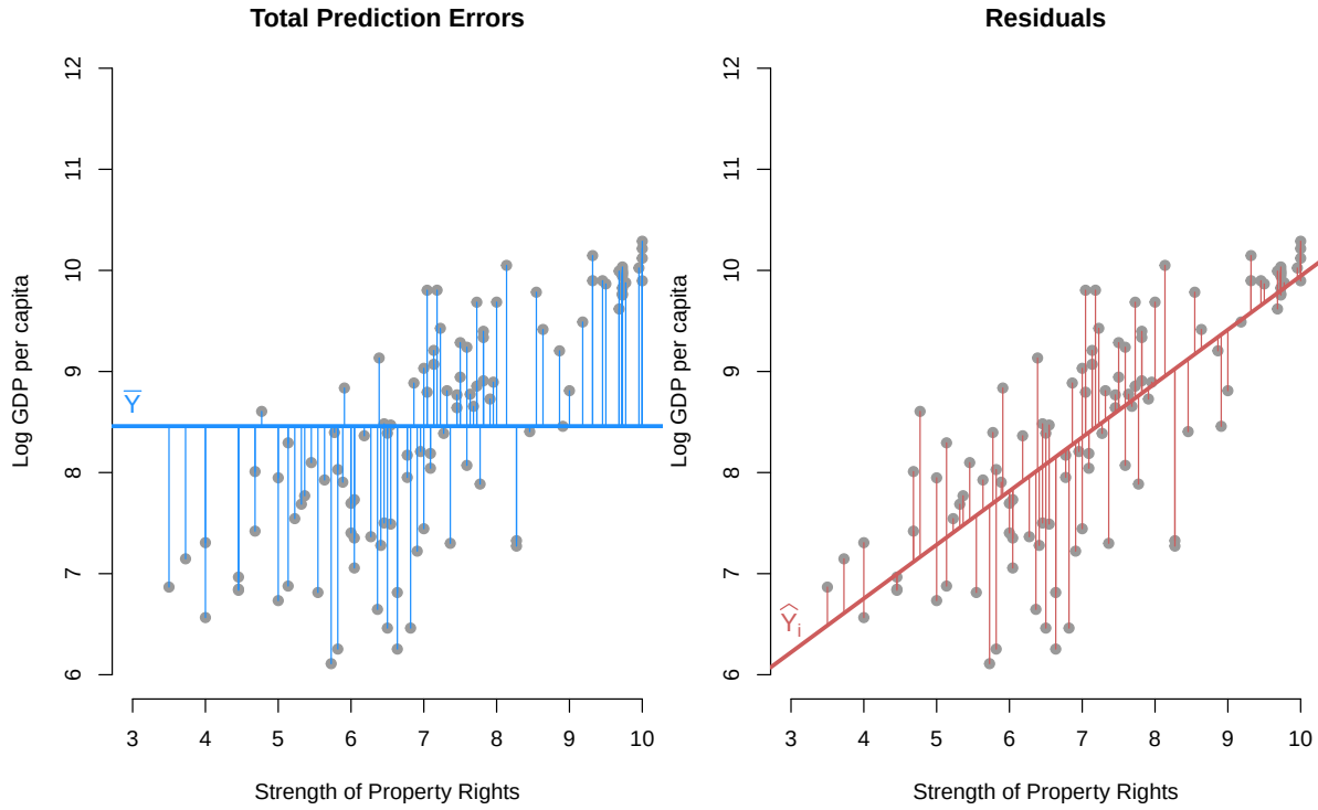
Figure 6.3: Total sum of squares vs. the sum of squared residuals.
