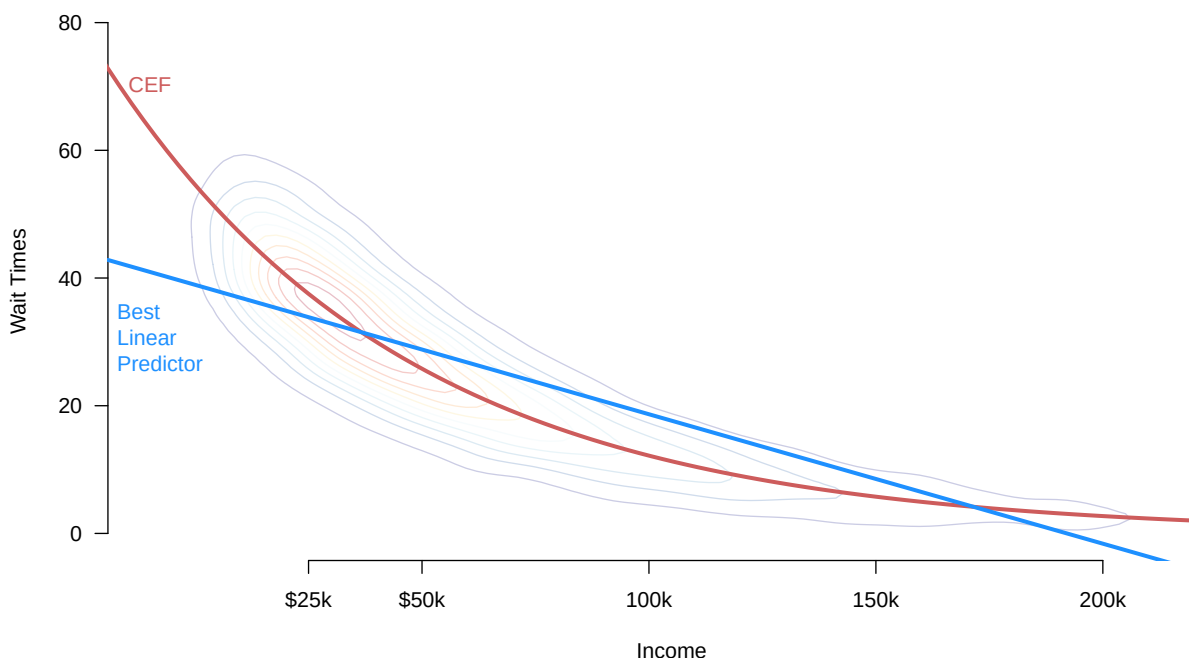
Figure 5.2: Comparison of the CEF and the best linear predictor.
