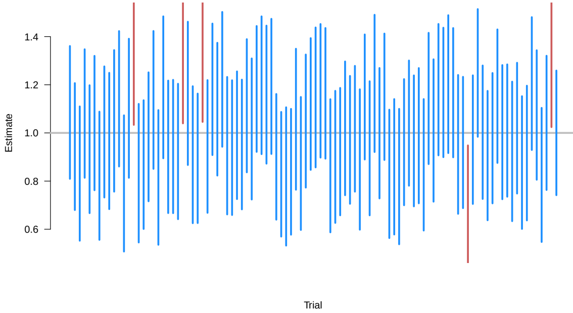
Figure 3.4: 95% confidence intervals from 100 random samples. Intervals are blue if they contain the truth and red if they do not.
