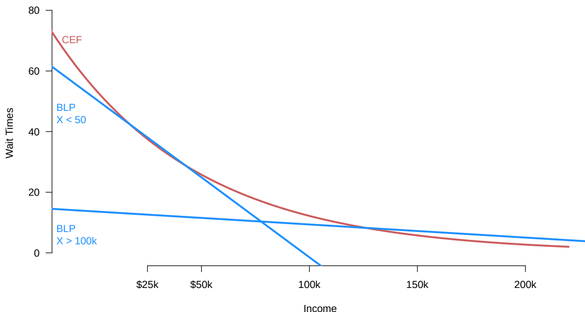
Figure 5.3: Linear projections for when truncating income distribution below $50k and above $100k.
