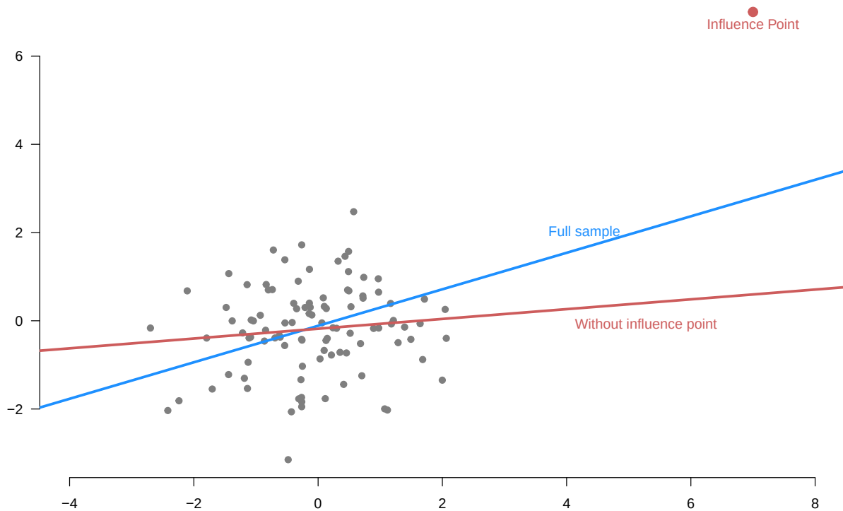
Figure 6.6: An example of an influence point.
