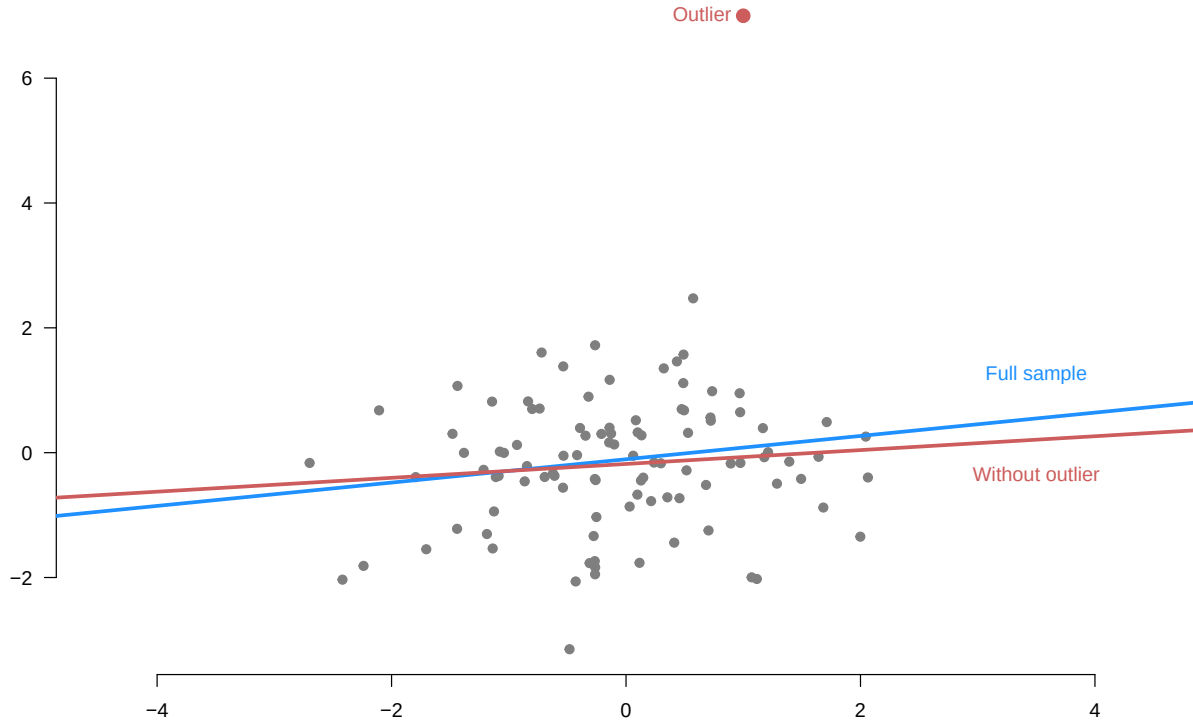
Figure 6.5: An example of an outlier.
