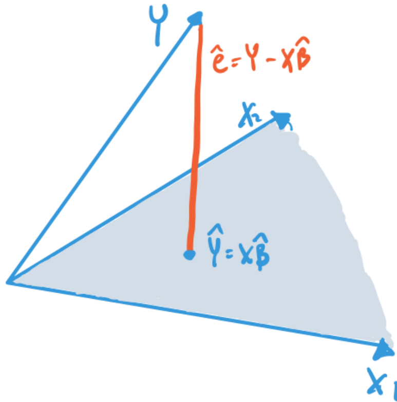
Figure 6.4: Projection of \mathbf{Y} on the column space of the covariates.
