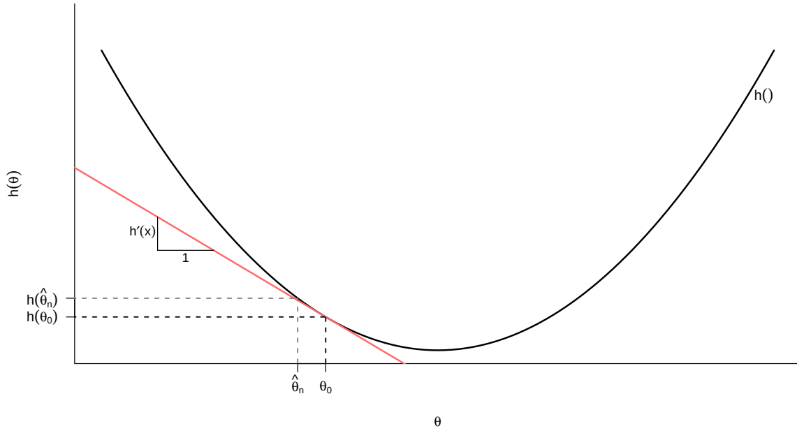
Figure 3.5: Linear approximation to nonlinear functions.
