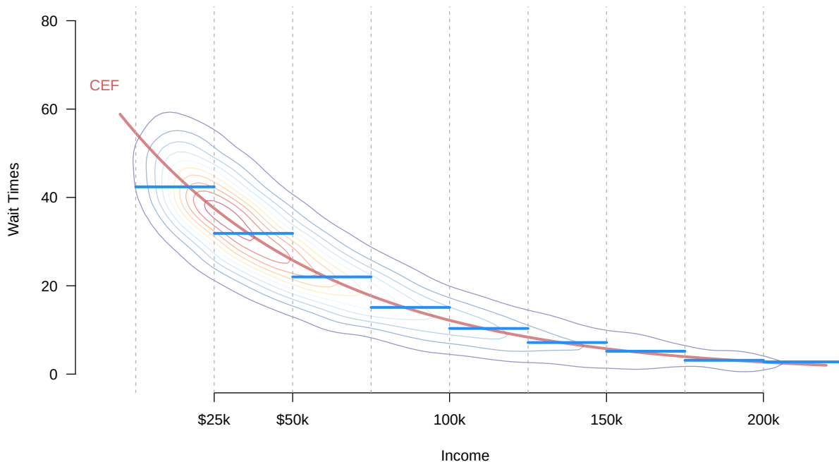
Figure 5.1: Hypothetical joint distribution of income and poll wait times (contour plot), conditional expectation function (red), and the conditional expectation of the binned income (blue).
