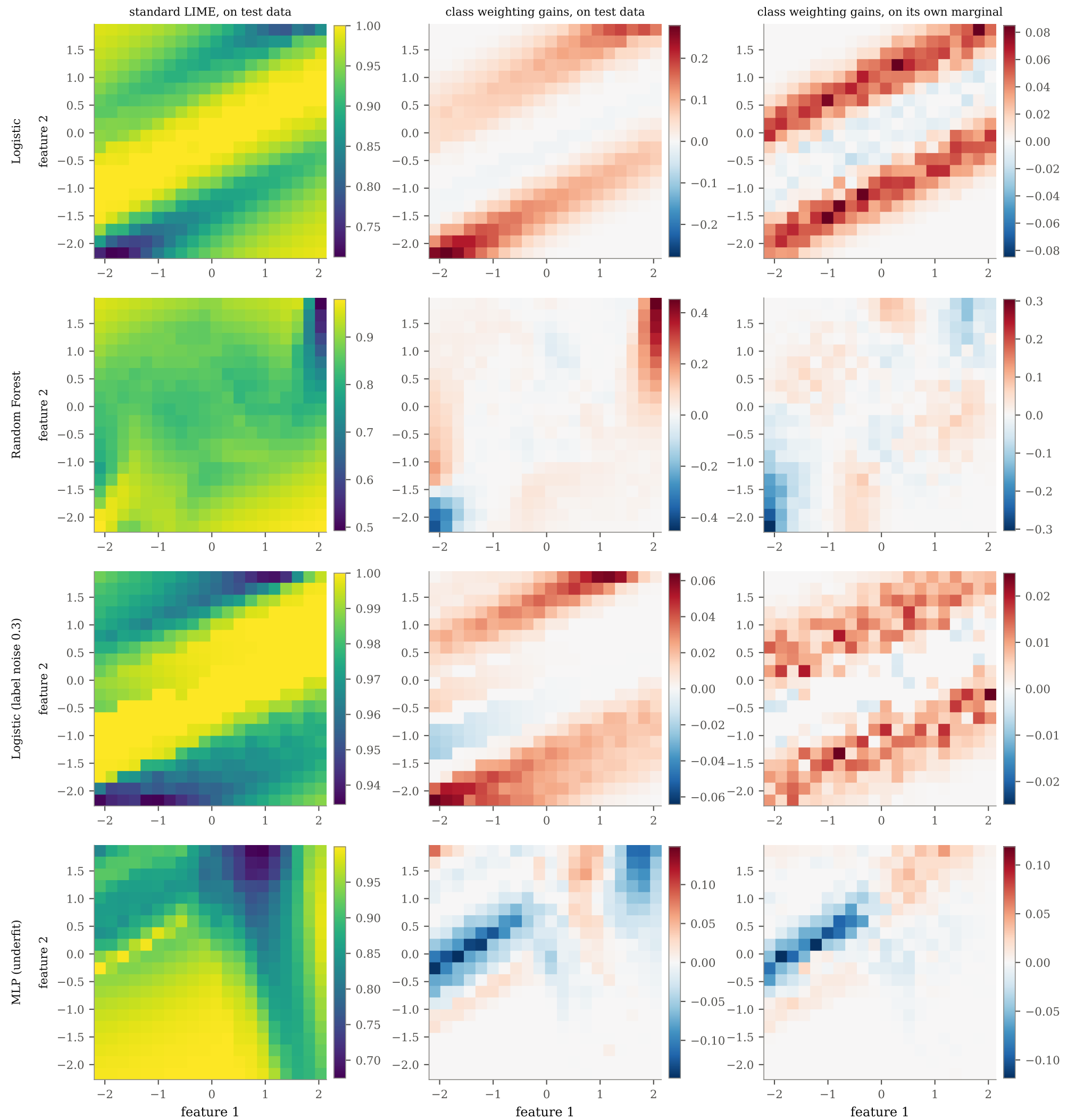
Moons: local fidelity over the grid, 400 query points per panel. Colour scales are per panel: the gains differ by an order of magnitude between black boxes
