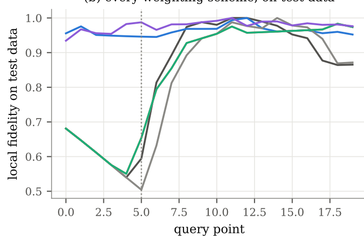
(b) every weighting scheme, on test data
