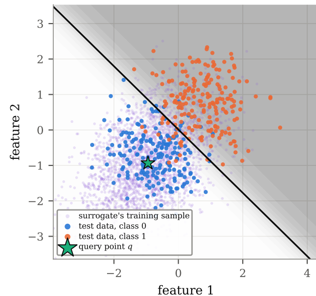
(a) trained on one distribution, judged against another
