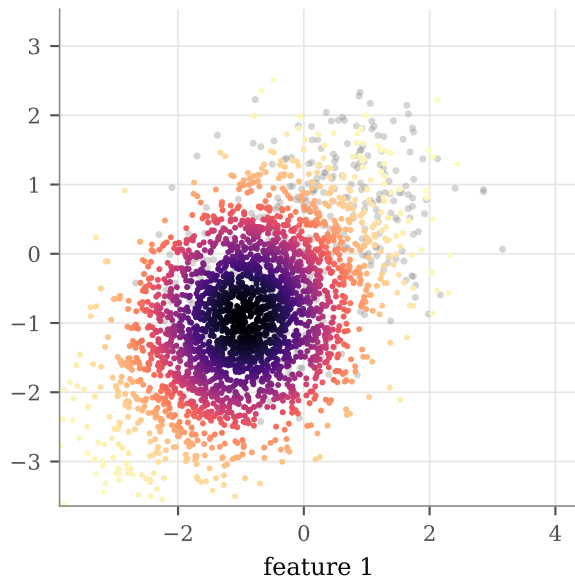
(b) locality kernel standard LIME
