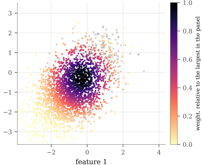
(d) \times density ratio pulls weight back towards the data
