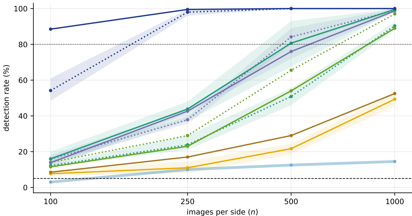
(a) CIFAR-10 vs CIFAR-100: the featuriser ladder, 200 repeats per cell
