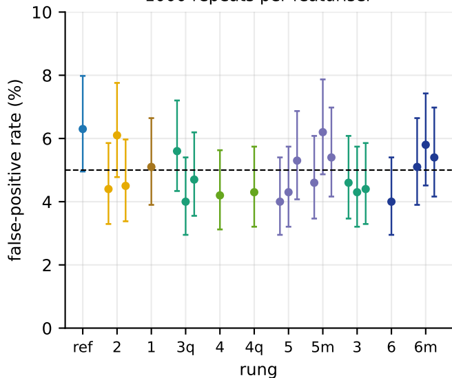
(c) calibration: redrawn null, n = 1000 1000 repeats per featuriser
