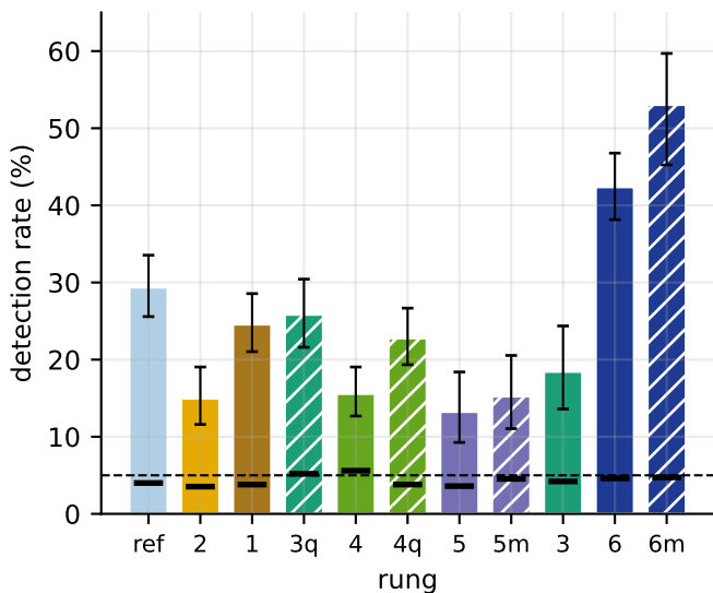
(b) drop 1 of 10 classes, n = 2000 bar = k = 9 , tick = k = 10 null
