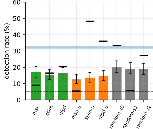
(c) drop 1 of 10 classes, n = 2000 bar = 64-D, tick = scalar
