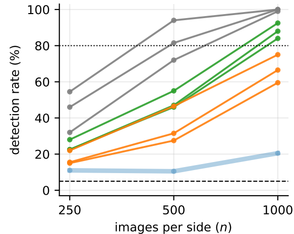
(a) CIFAR-10 vs CIFAR-100 64-D C2ST, 200 repeats
