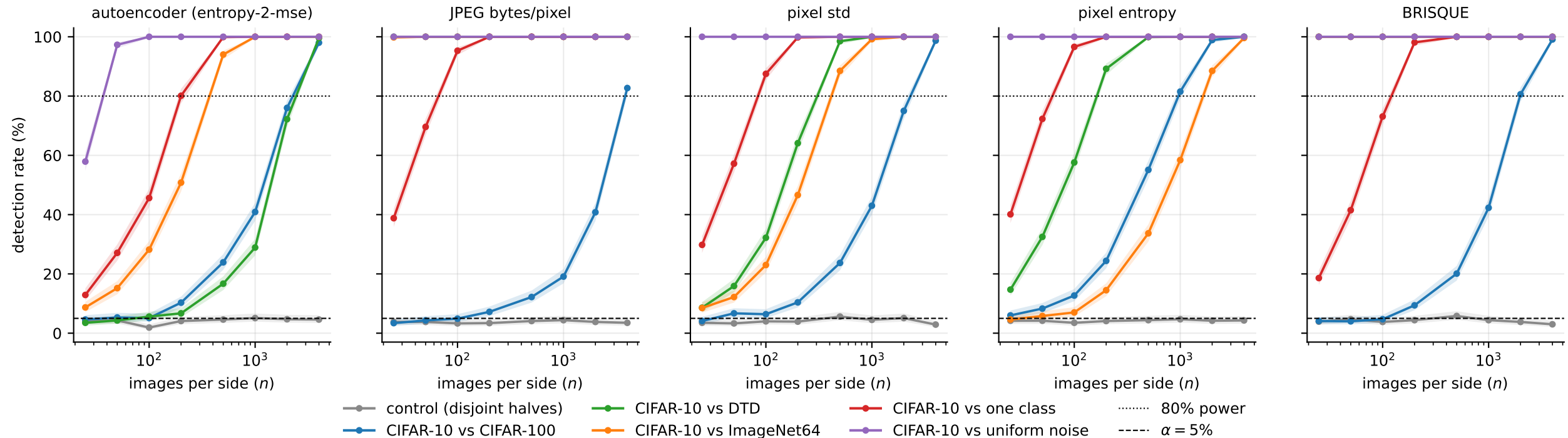
How many images before the test notices?
