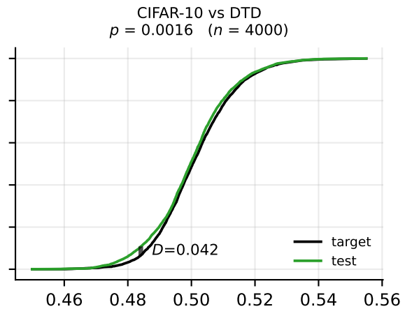
Score distributions as ECDFs -- autoencoder (entropy-2-mse) at 256px. The bar is the KS statistic.
