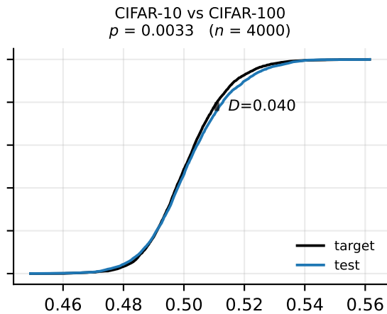
Score distributions as ECDFs -- autoencoder (entropy-2-mse) at 256px. The bar is the KS statistic.
