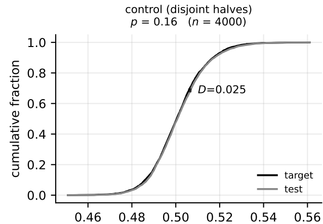
Score distributions as ECDFs -- autoencoder (entropy-2-mse) at 256px. The bar is the KS statistic.
