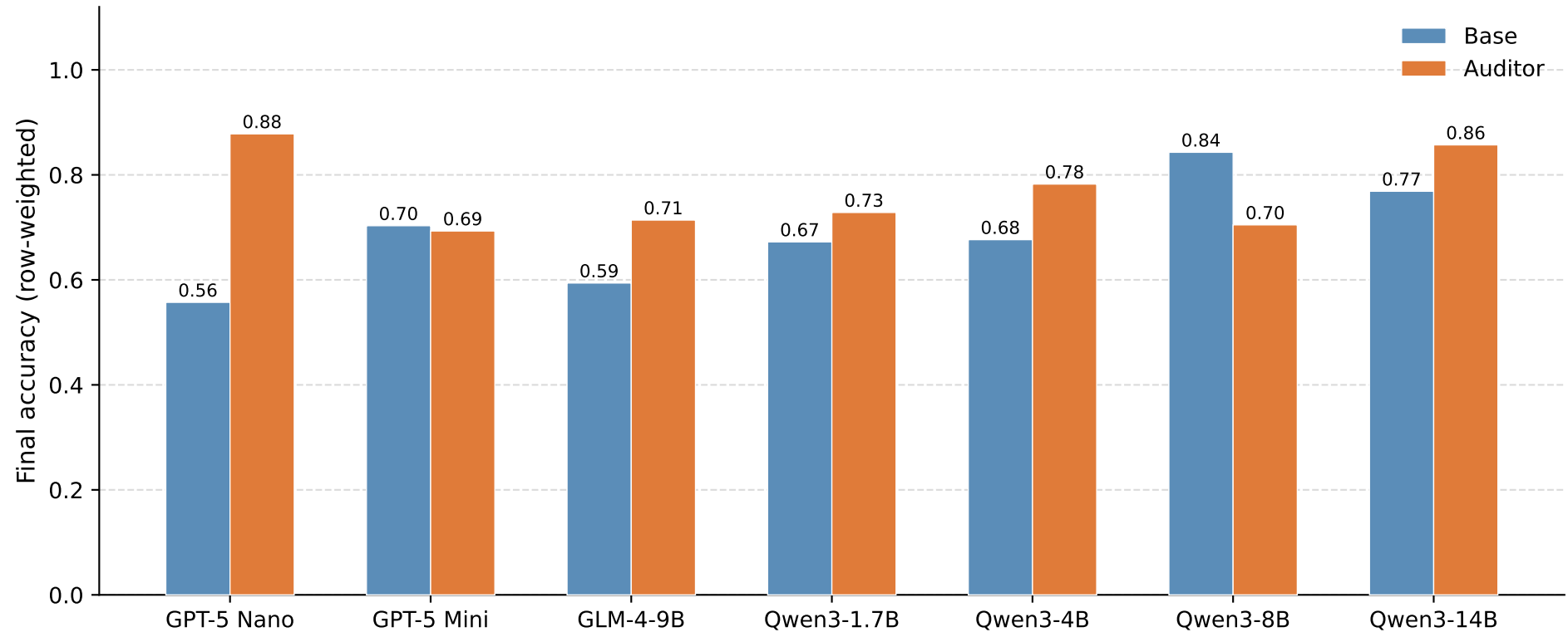
Final Accuracy by Model and Reasoning Method
