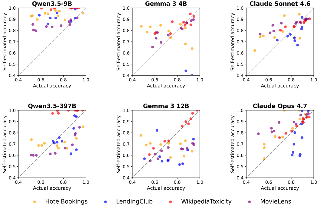
Figure 4: Most models overestimate their own accuracy. Actual versus self-estimated accuracy for each model across four datasets. Points above the diagonal indicate overconfidence (self-estimated > actual). Across 304 model \times condition pairs, 201 (66%) are overconfident. The direction of miscalibration varies by model: some are predominantly overconfident, others underconfident.
