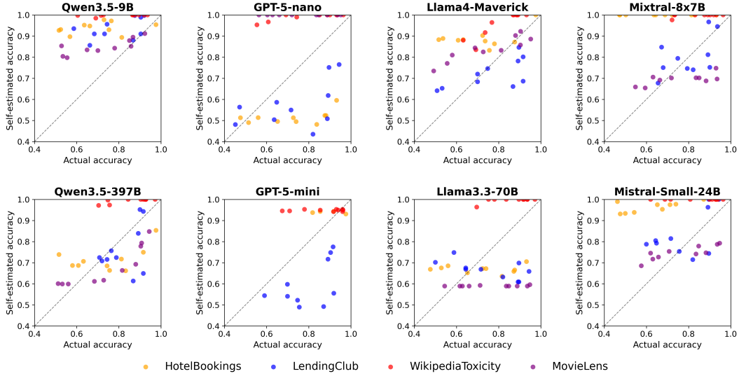
Figure 4: Most models overestimate their own accuracy. Actual versus self-estimated accuracy for each model across four datasets. Points above the diagonal indicate overconfidence (self-estimated > actual). Across 304 model \times condition pairs, 201 (66%) are overconfident. The direction of miscalibration varies by model: some are predominantly overconfident, others underconfident.
