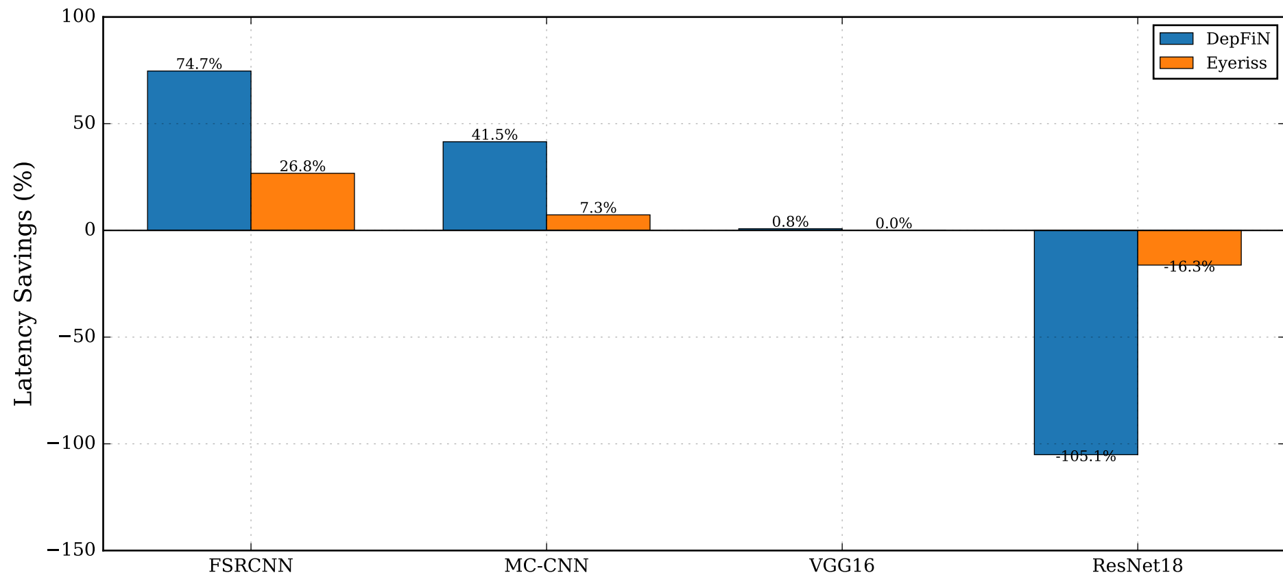
Auto-Sized Fusion — Latency Savings (Full vs Single)
