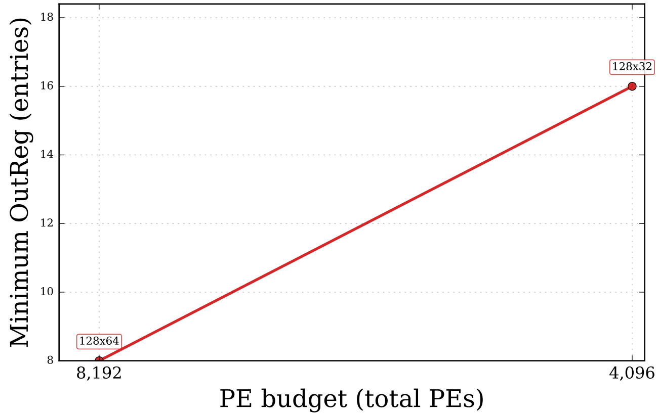
ResNet18
