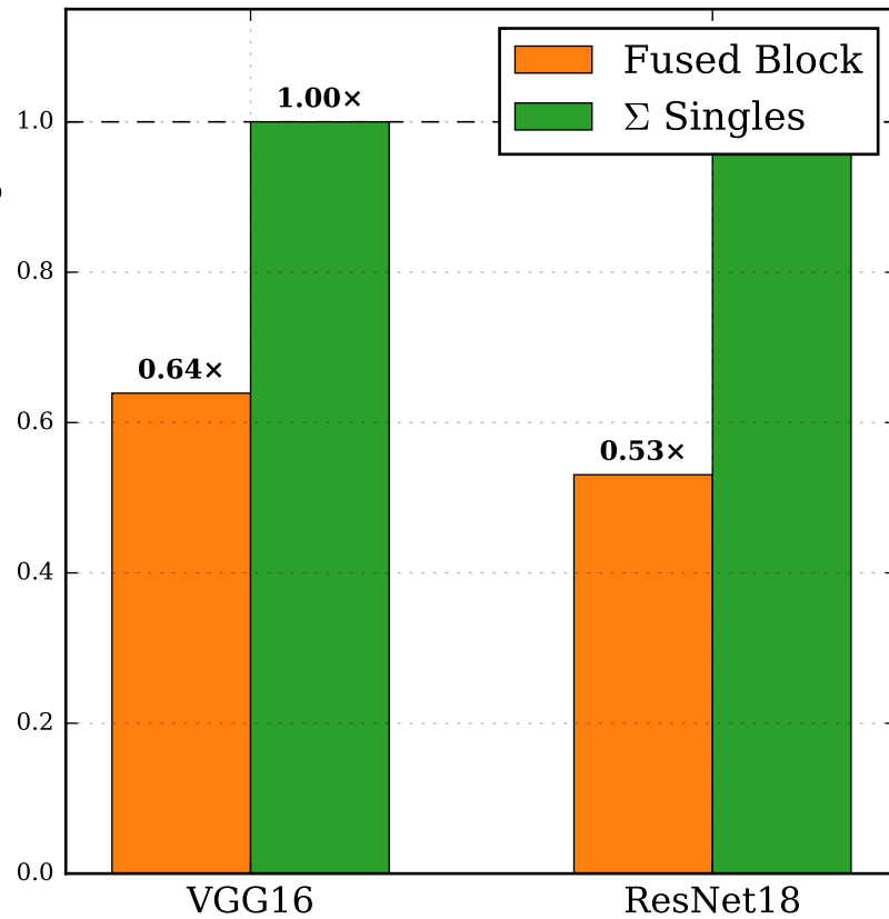
Normalised Latency
