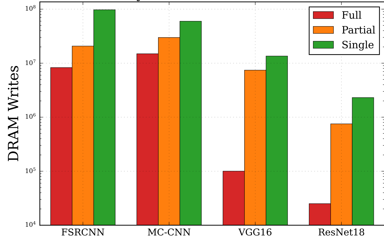
Eyeriss — DRAM Writes
